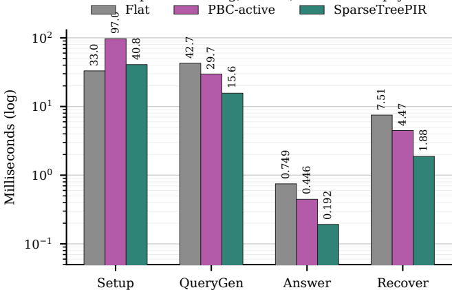
SimplePIR timing, h = 24 , 99.95\% empty
