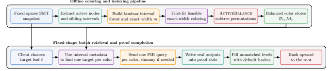
Fig. 3. End-to-end view. The server partitions only active proof-bearing nodes into color subdatabases, while the client retrieves at most one real node per color and completes the remaining proof levels from public default hashes.
