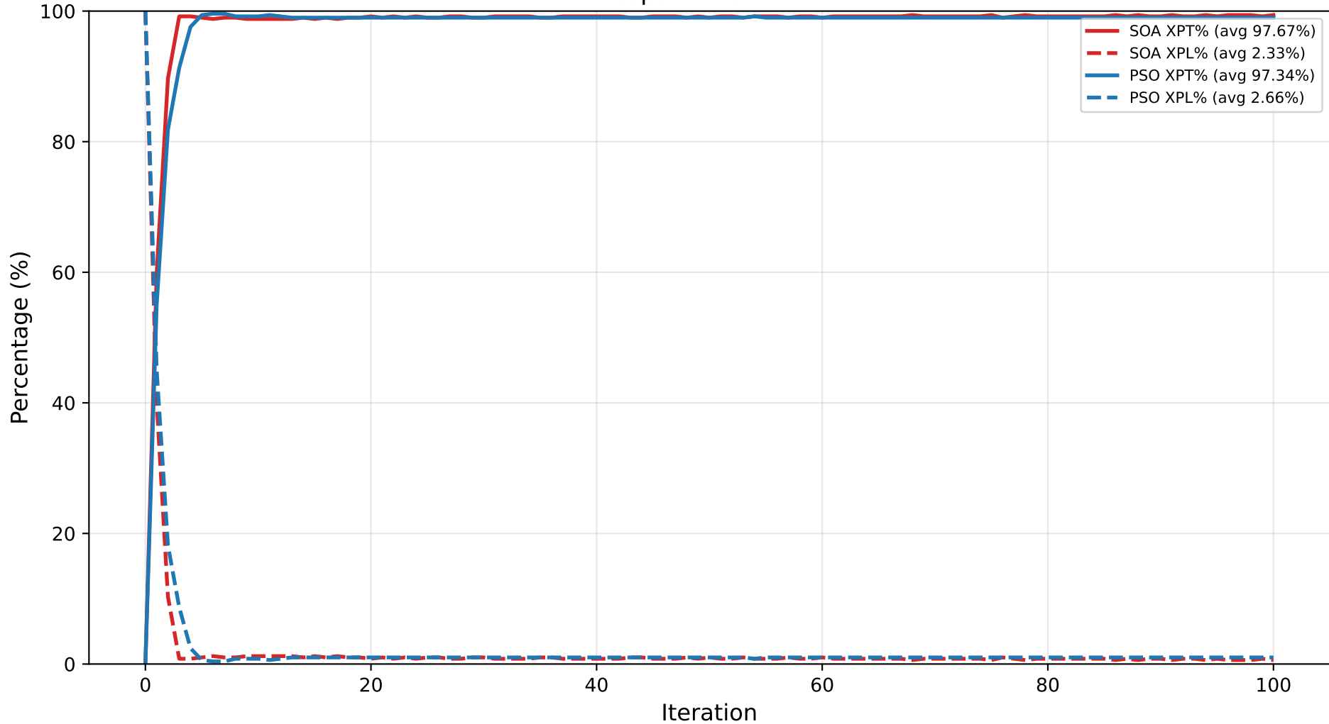
Exploration (XPL) vs Exploitation (XPT) per MH scp64 - V3-ELIT
