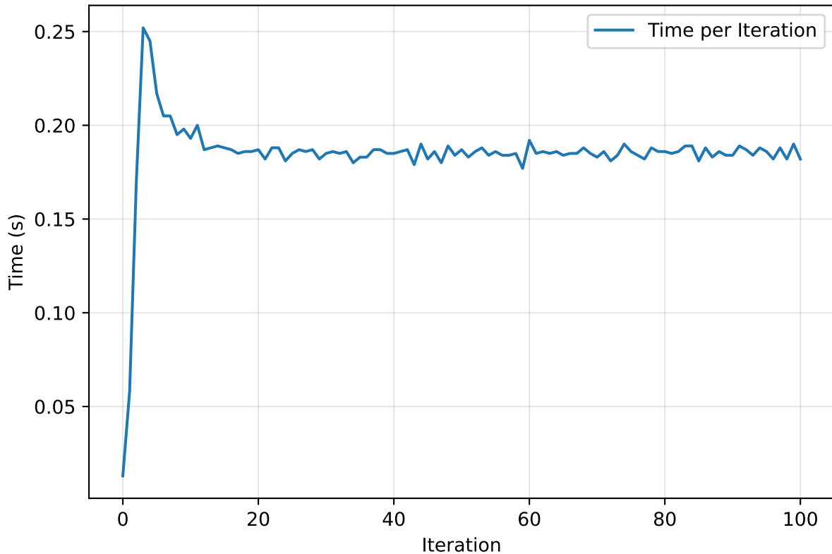
Time per Iteration PSO scp64 - Run 2 - (V3-ELIT)
