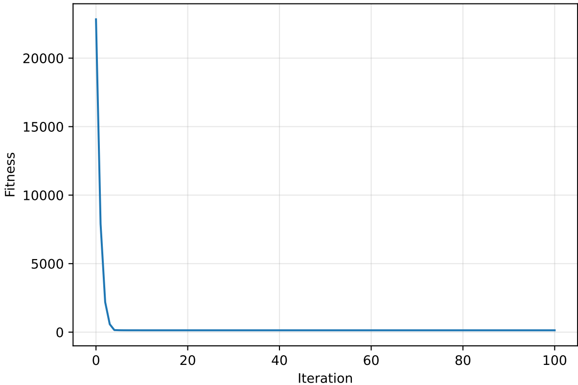
Convergence PSO scp64 - Run 2 - (V3-ELIT_LOG)
