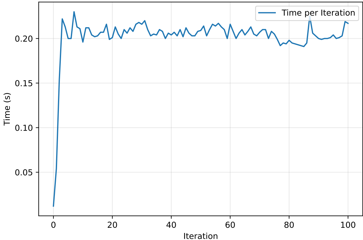
Time per Iteration PSO scp64 - Run 2 - (V3-ELIT_LOG)
