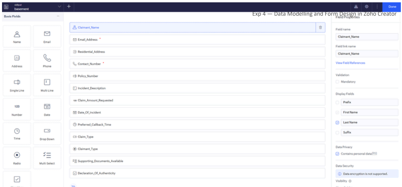
Fig. 2 — Zoho Creator form builder: field palette, form fields, and field properties panel
