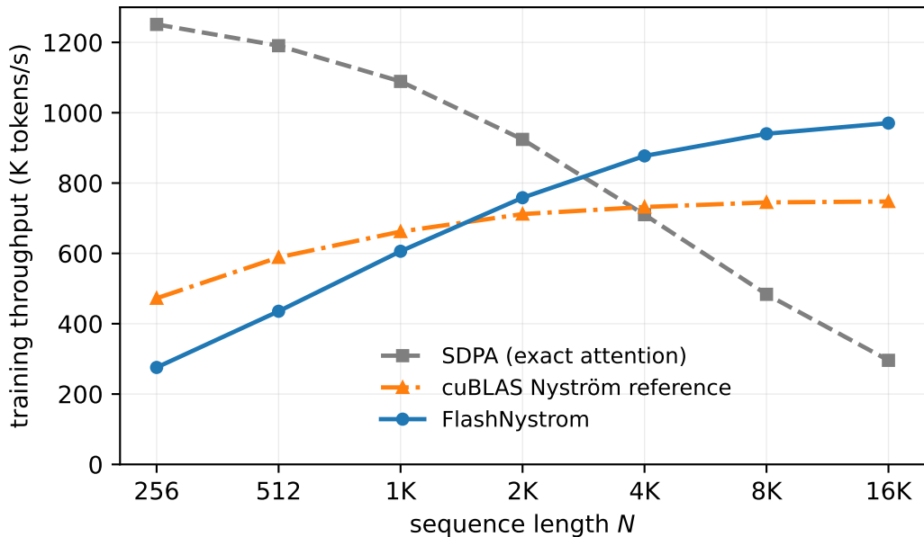
fwd+bwd, FP16, largest fitting batch (NVIDIA A100-SXM4-40GB)
