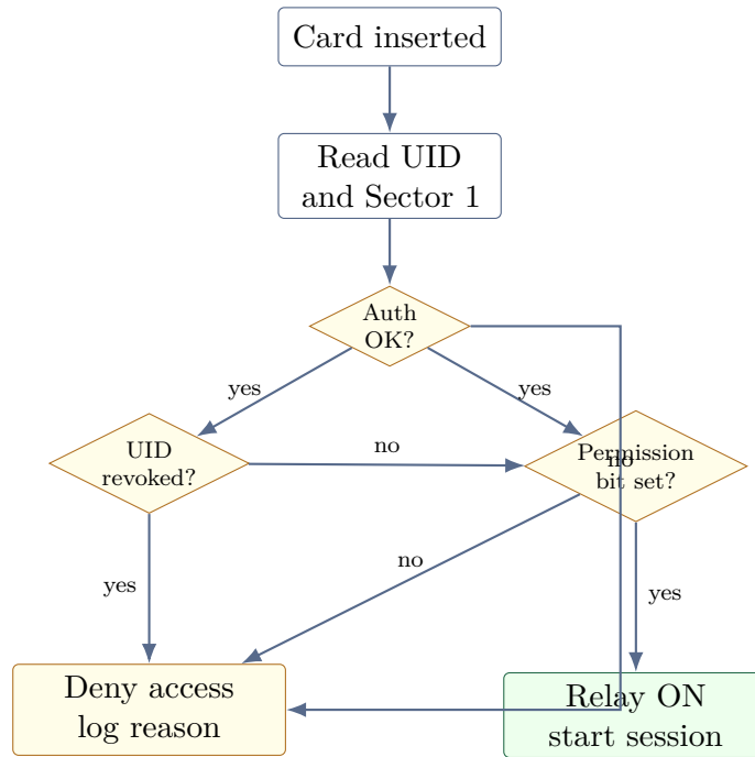
Figure 4.3: Offline access validation flow
