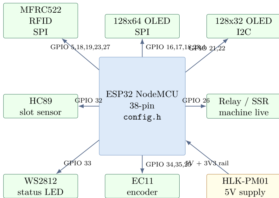
Figure G.1: Access node wiring overview
