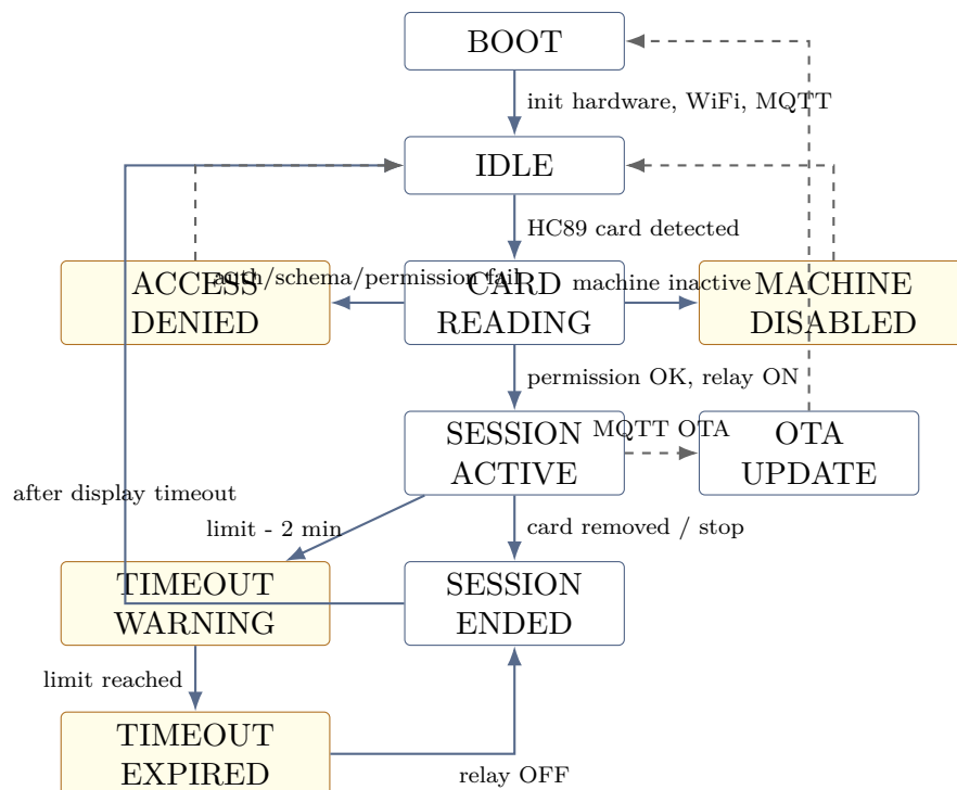
Figure 7.1: Access Node Firmware State Machine
