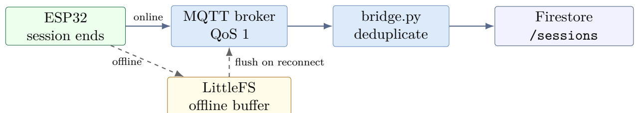
Figure 4.4: Session logging and offline sync path
