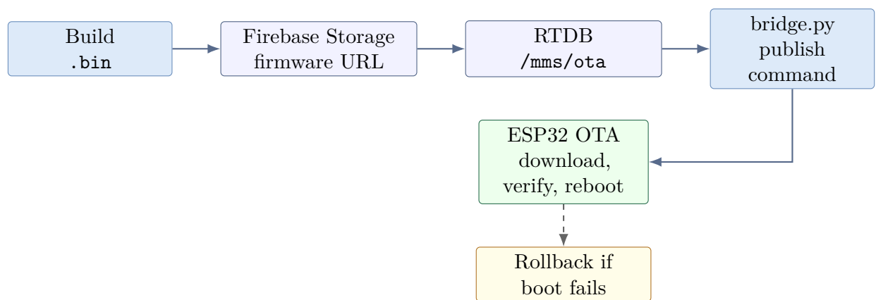
Figure 4.7: OTA release flow
