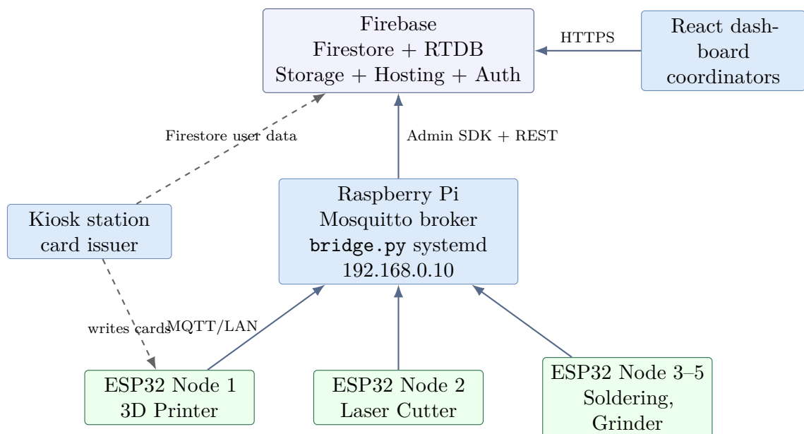
Figure 4.1: MMS V2 System Architecture
