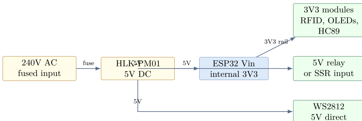
Figure G.2: Power distribution
