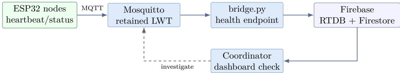
Figure 12.1: Monitoring chain and human response loop
