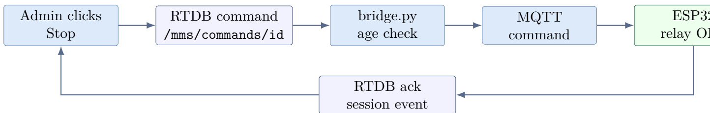
Figure 4.5: Remote stop command path
