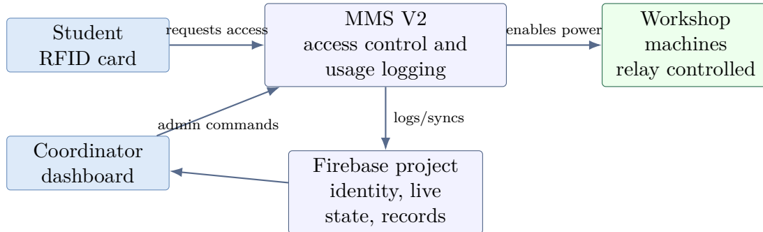
Figure 4.2: System context diagram
