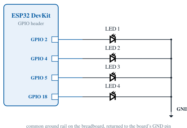
Figure 4: Circuit schematic for Experiment 2. The topology is identical to Figure 1; only the driving pins change.
