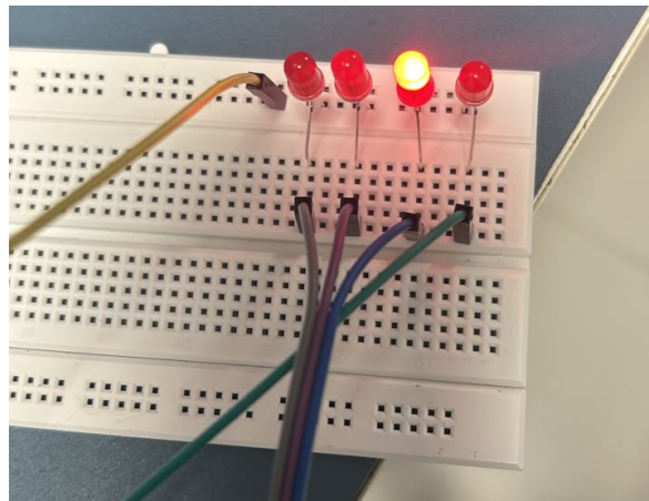
Figure 3: Experiment 1 — the four LEDs on the breadboard during the blink cycle, with the jumper wires running to the GPIO header and all cathodes on the common ground rail.
