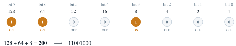
Figure 7: Place values of the eight LEDs and the pattern displayed for the input 200. The same mapping was confirmed on the serial monitor for the inputs 20 \rightarrow 00010100 and 25 \rightarrow 00011001 .
