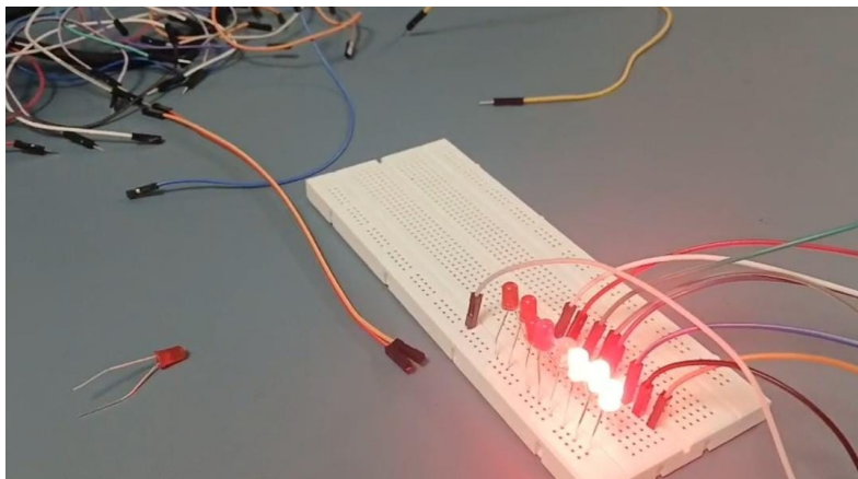
Figure 6: The assembled circuit — eight LEDs in a row on the breadboard, each wired directly to its own GPIO pin, with the cathodes on the common ground rail.
