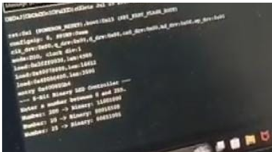
Figure 4: Three further outputs, taken on the ESP32 cross-check: Output 3 200 \rightarrow 11001000 , Output 4 20 \rightarrow 00010100 and Output 5 25 \rightarrow 00011001 . Each printed string matched the pattern of lit LEDs on the breadboard.
