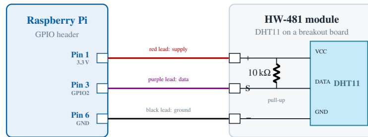
Figure 2: Circuit schematic. The HW-481 module needs only supply, ground and one data line; its on-board 10 kΩ resistor holds the data line HIGH when neither side is driving it.
