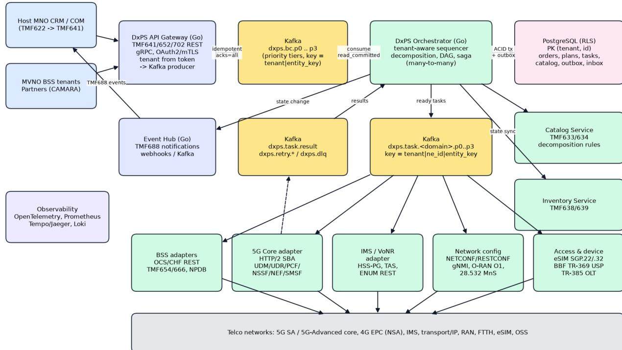
Figure: DxPS logical architecture
