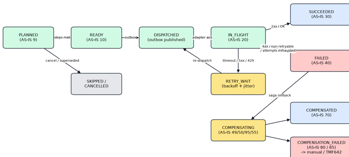
Figure 6 - NE task state machine
