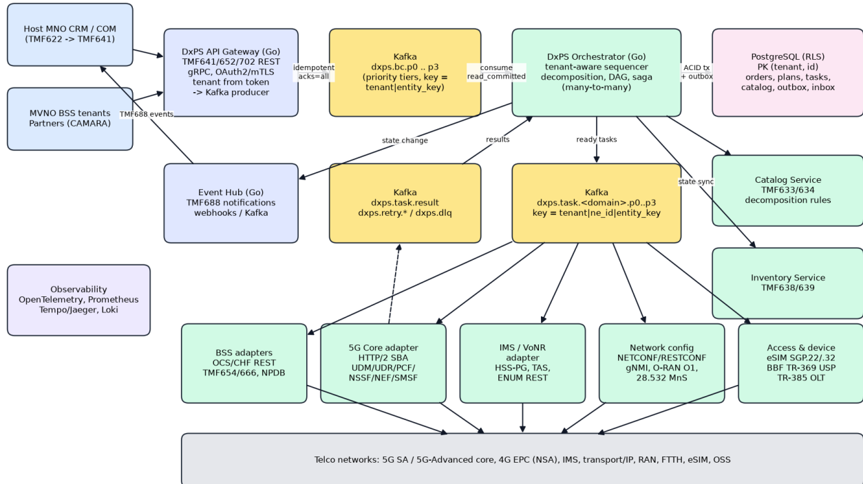
Figure 2 - DxPS logical architecture
