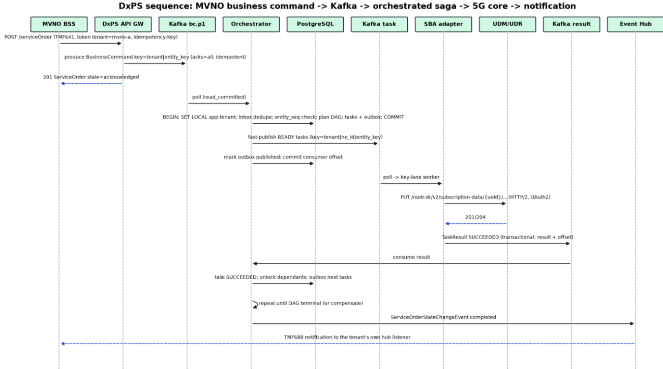
Figure 5 - Activation sequence (happy path)
