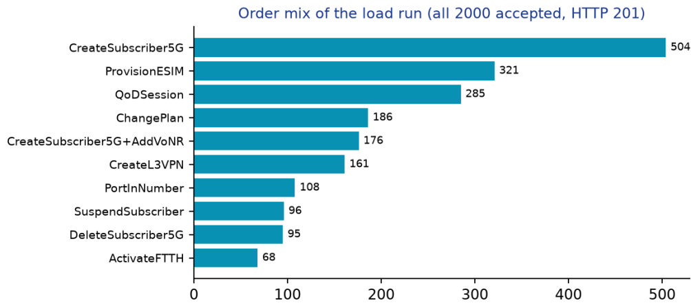
Figure 3 - Order mix of the load run
