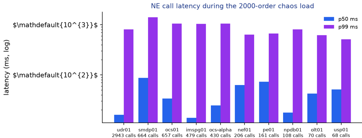
Figure 4 - NE call latency (log scale); error counts include the injected chaos faults
