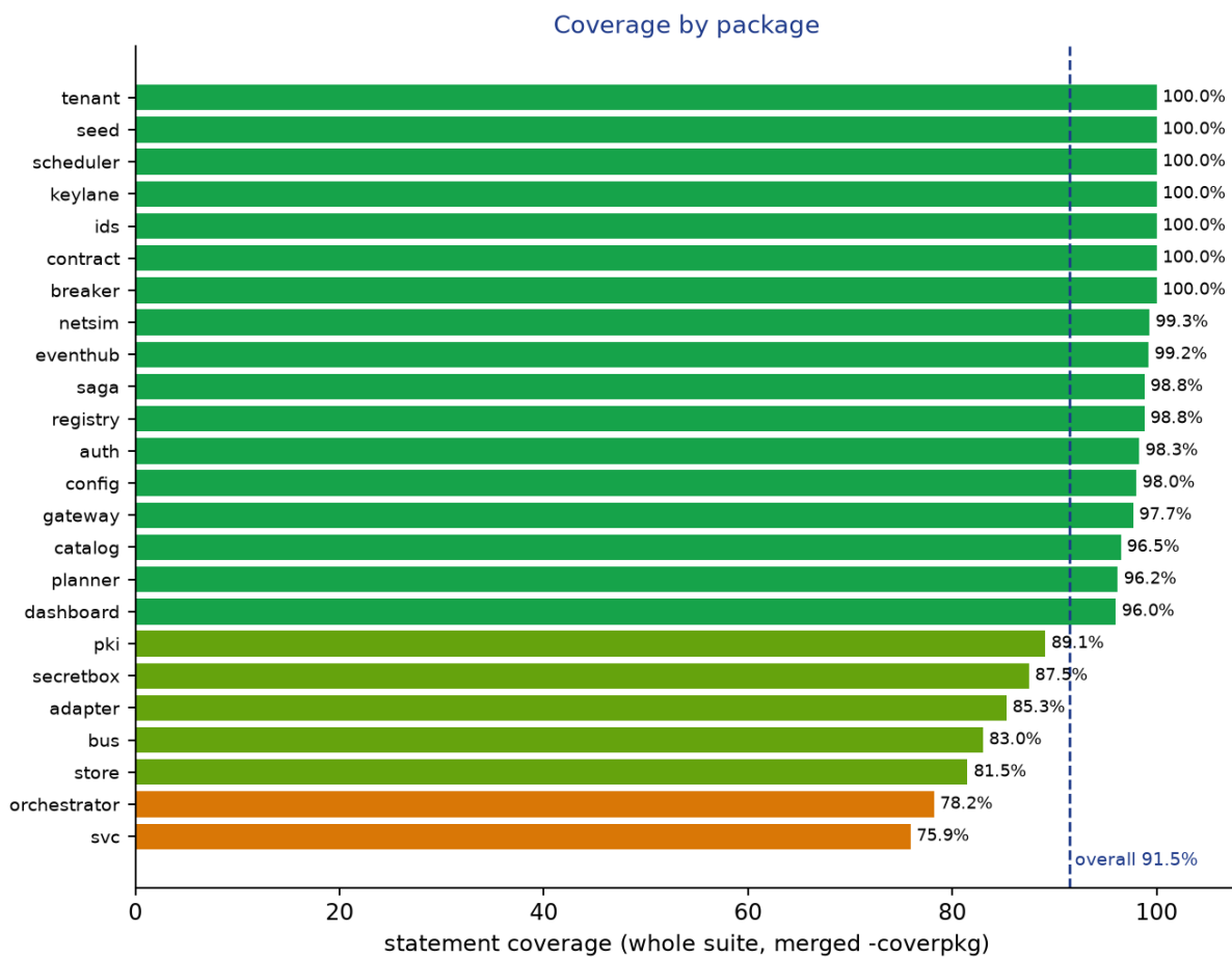
Figure 1 - Statement coverage per package (whole suite)
