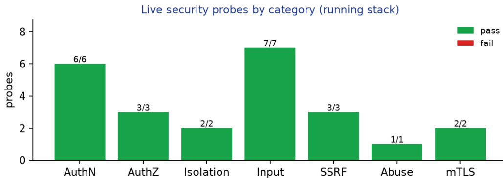
Figure 2 - Live security probes by category
