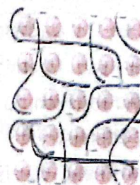
Electrons moving between the cations
