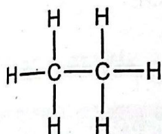
Ethane
