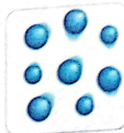
Gases
