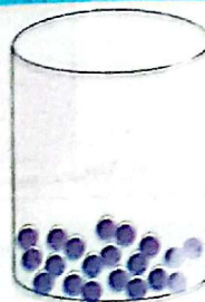
Liquid
