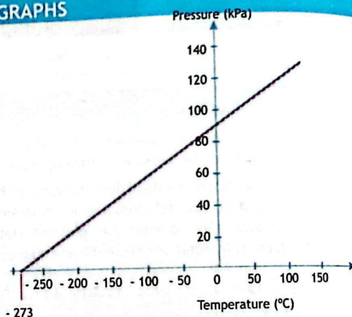
(b) Graph between temperature and pressure of a substance showing absolute zero
