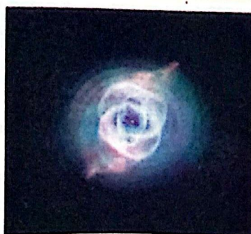
Nebula
