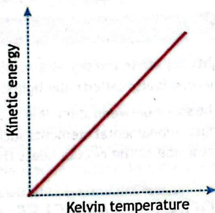
(a) Graph between temperature and kinetic energy of particles
