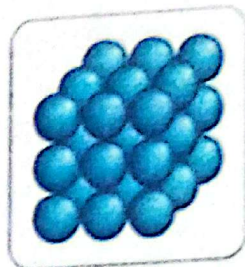
Solids
