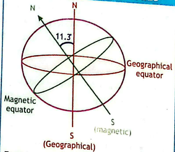
FIGURE 8.20 EARTH'S POLES
