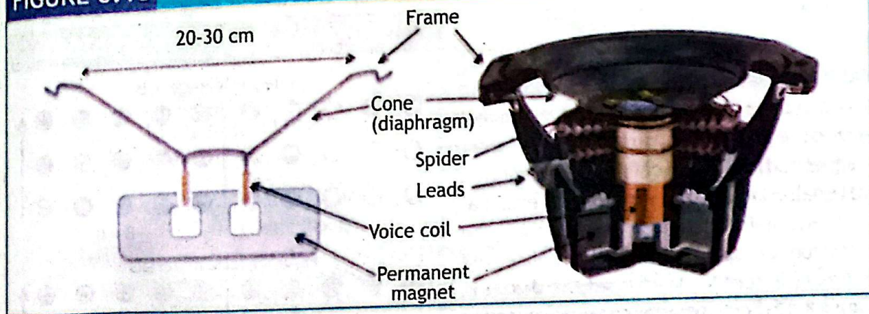
FIGURE 8.15 ANATOMY OF SPEAKER
