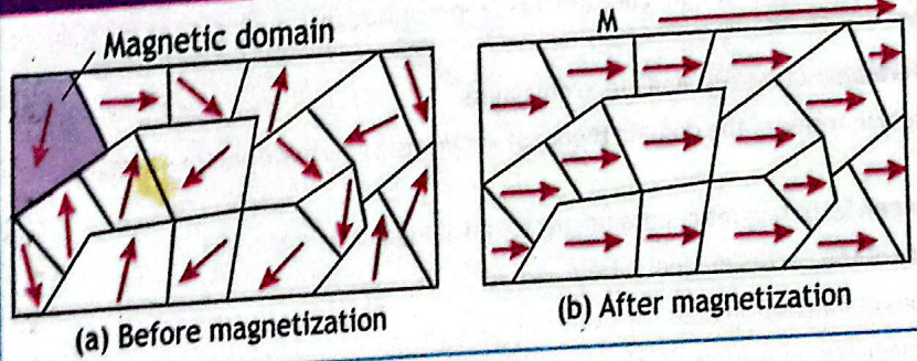
FIGURE 8.2 DOMAINS
