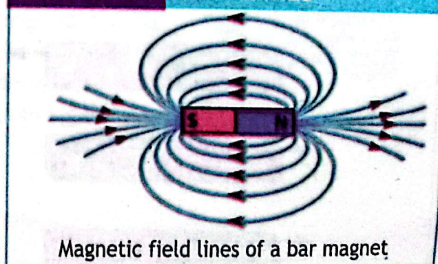
FIGURE 8.4 FIELD LINES
