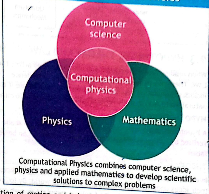
FIGURE 9.3 COMPUTATIONAL PHYSICS
