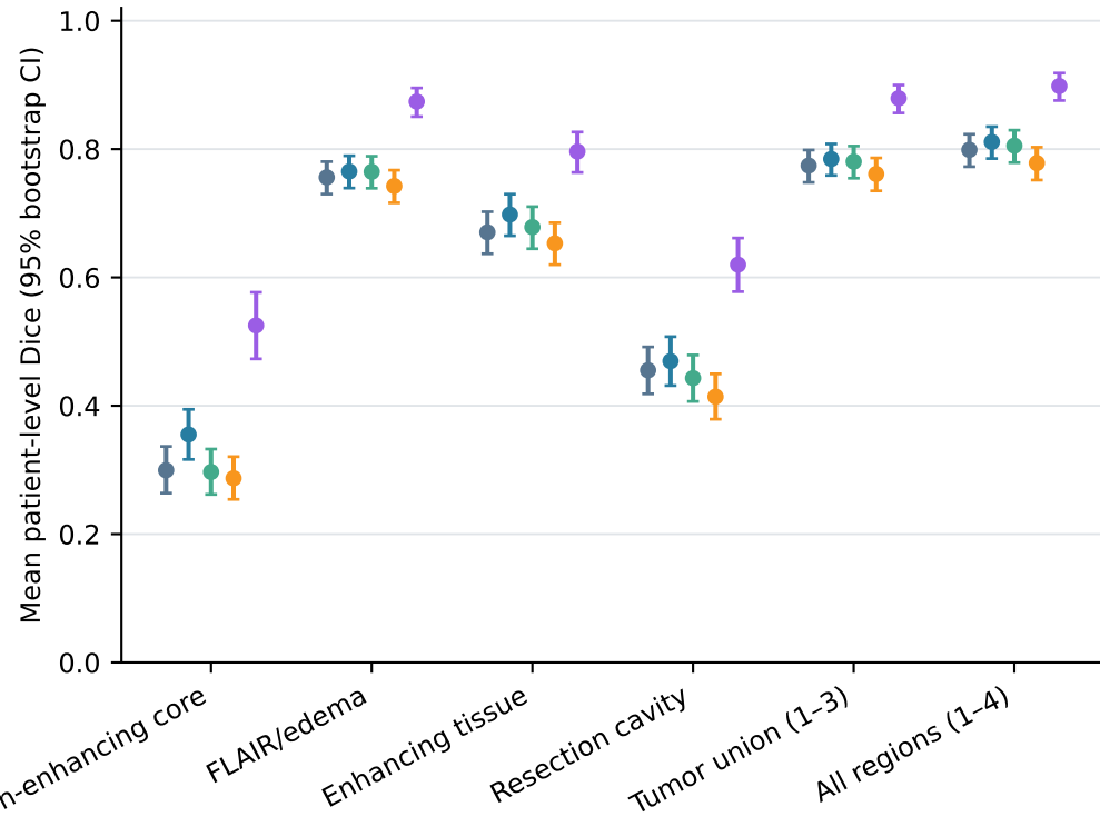
A Reference-present overlap
