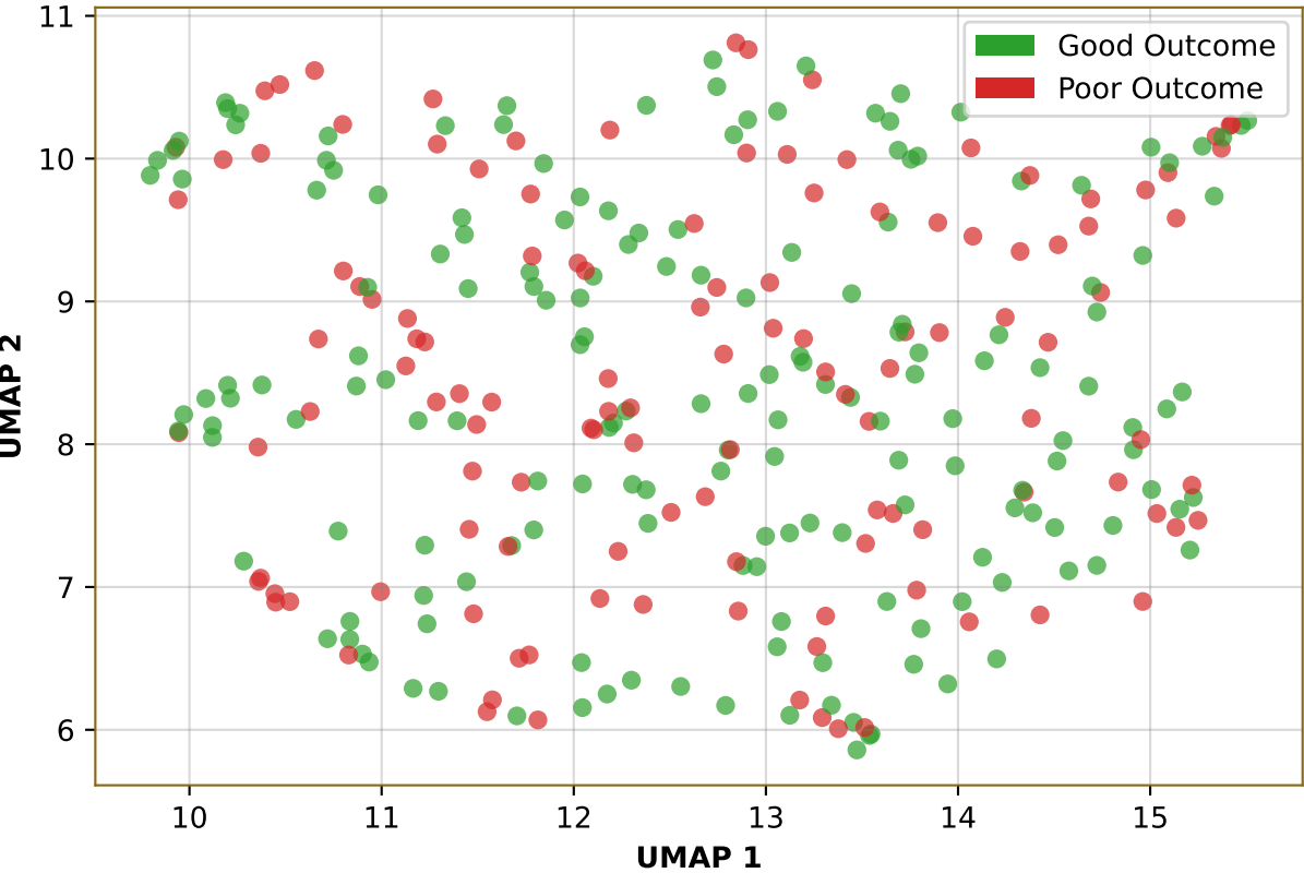
UMAP Analysis
