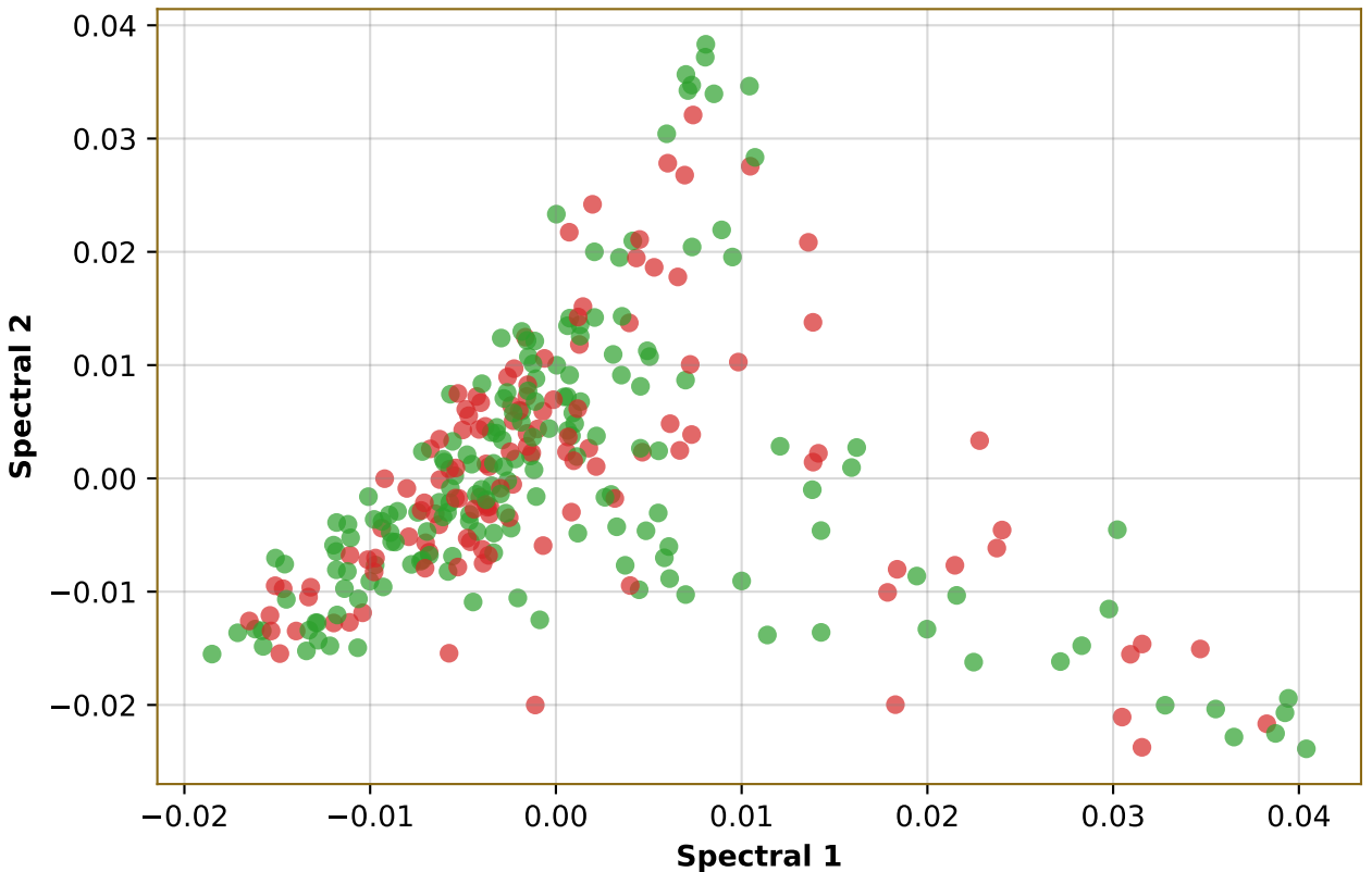
Spectral Embedding
