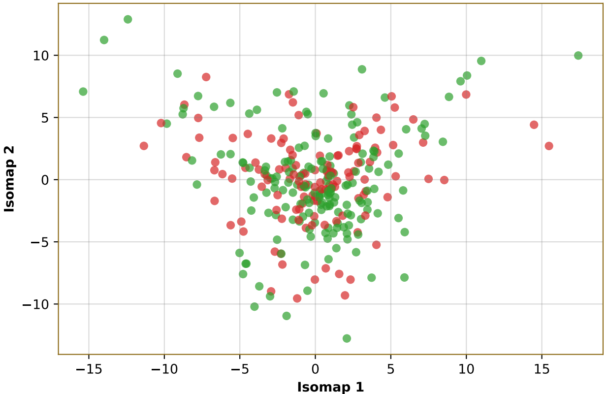
Isomap Analysis
