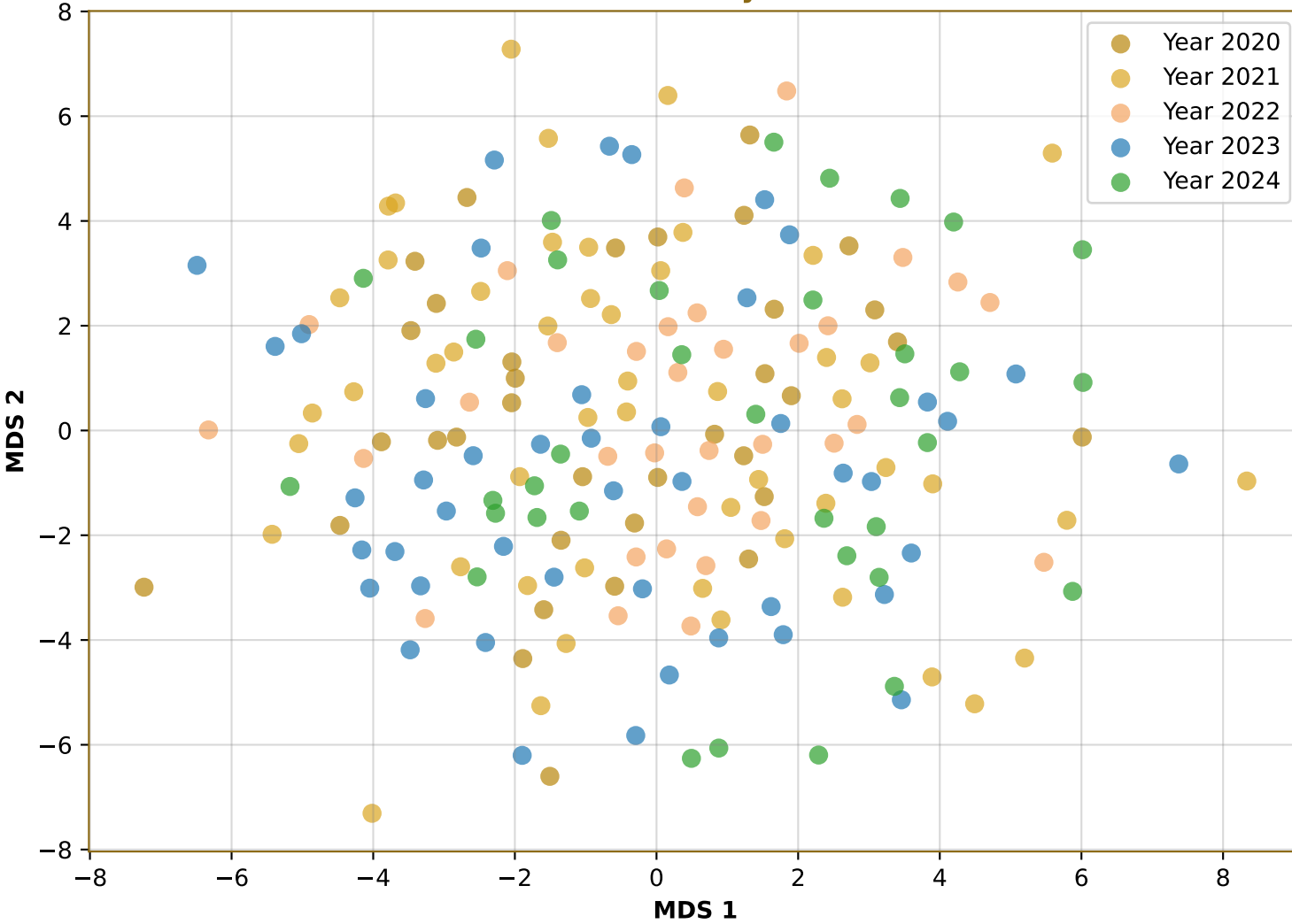
MDS Analysis
