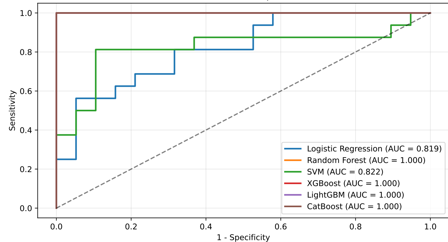
ROC Curves Comparison
