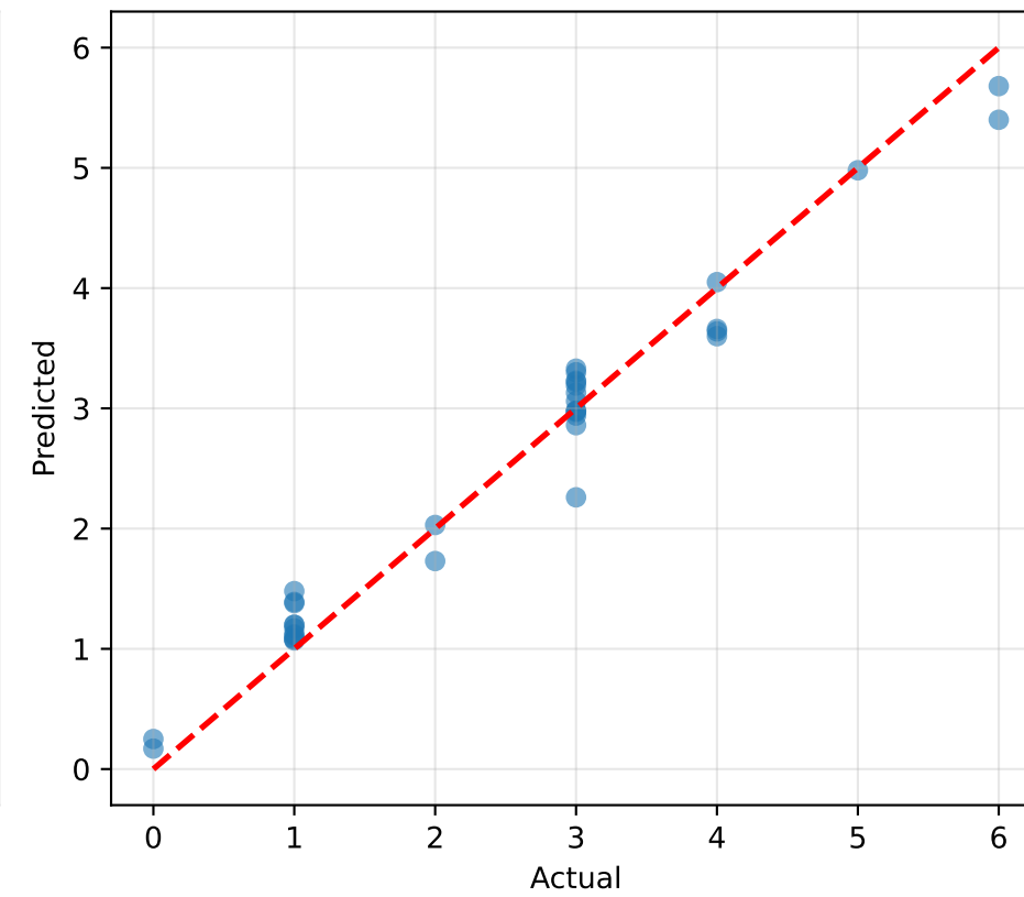
CatBoost MAE=0.348, R 2 =0.903
