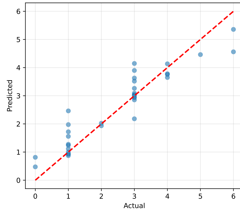
LightGBM MAE=0.408, R 2 =0.857
