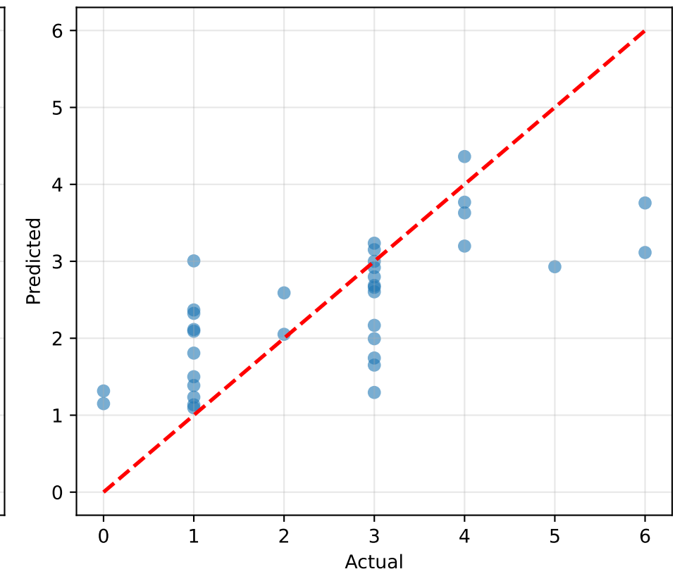
SVR MAE=0.828, R 2 =0.483
