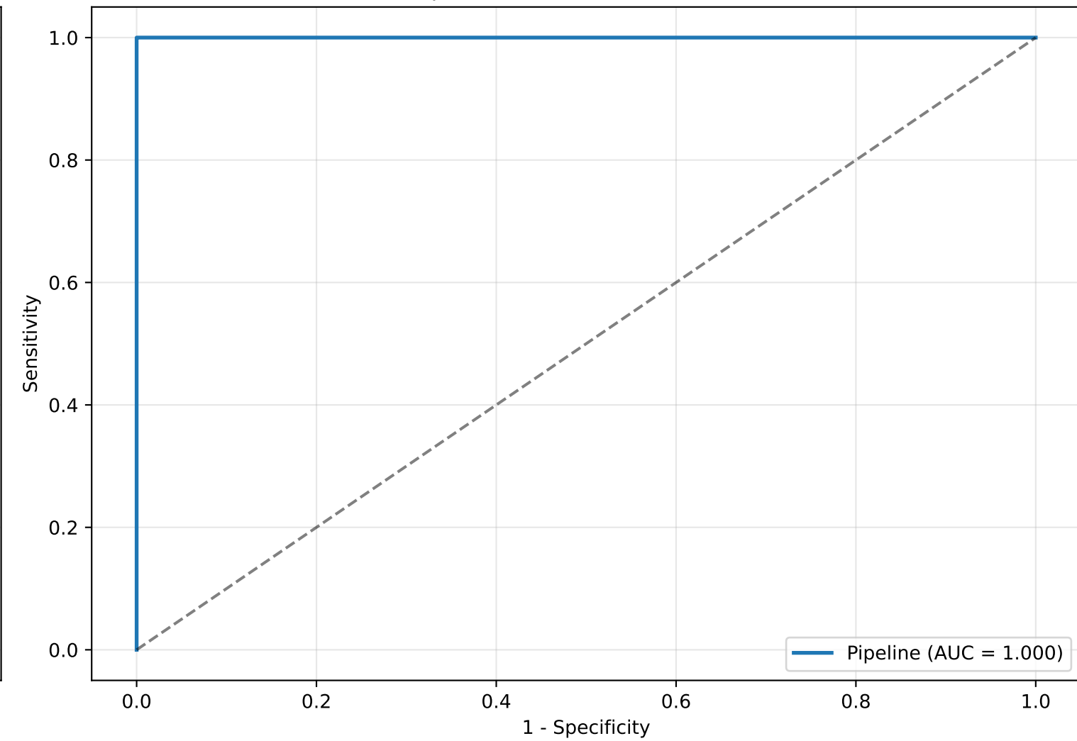
Advanced Models Performance
