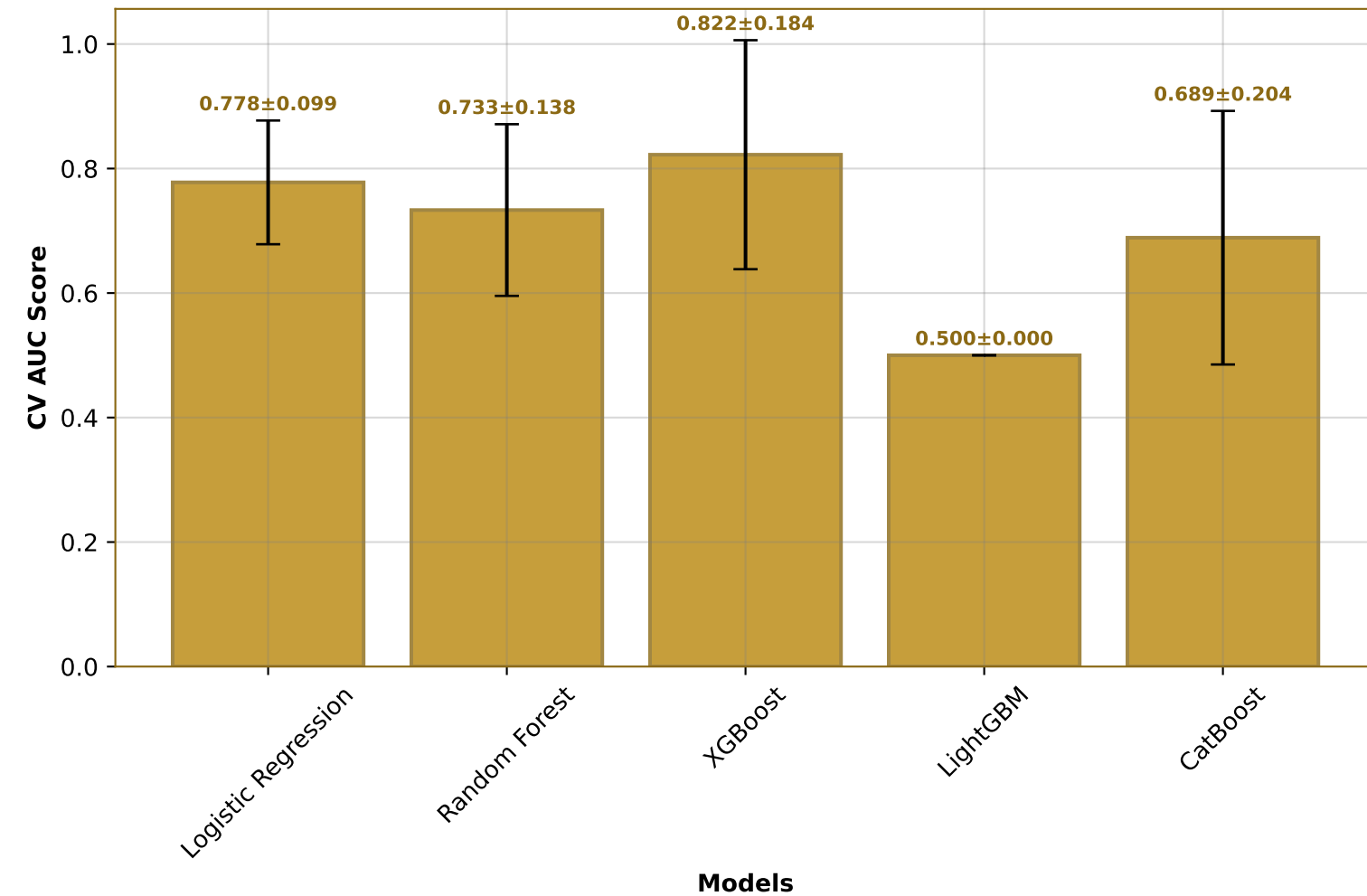
Cross-Validation Performance
