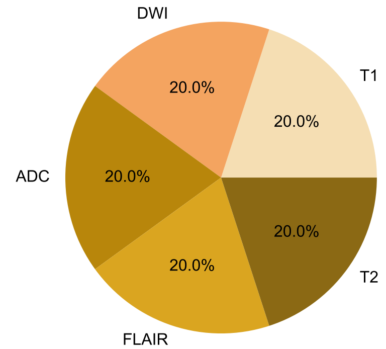
Modality Distribution
