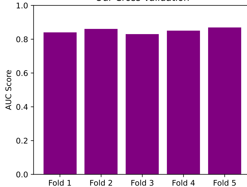
Our Cross-Validation
