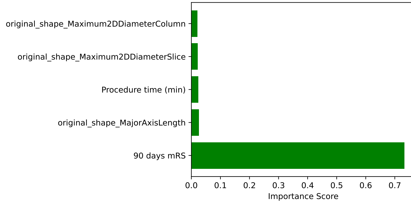
Our Cross-Validation
