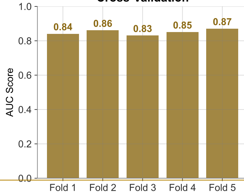
Cross-Validation
