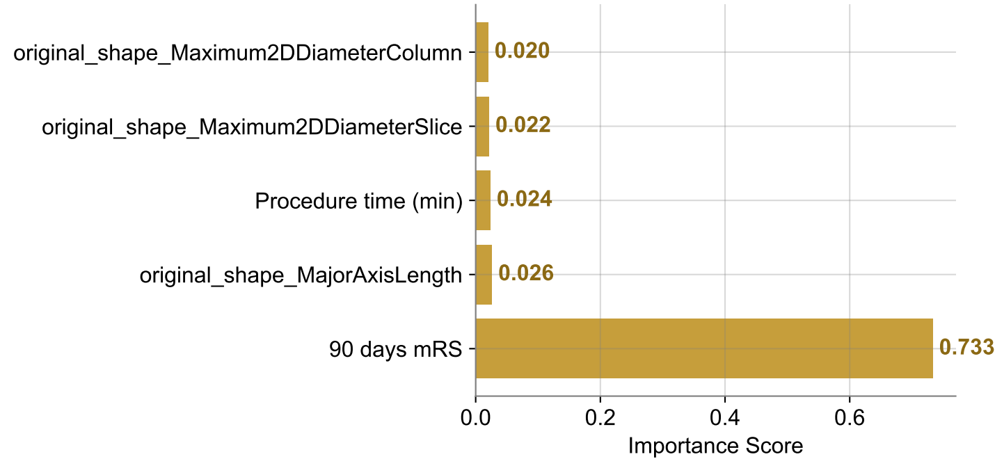
Cross-Validation
