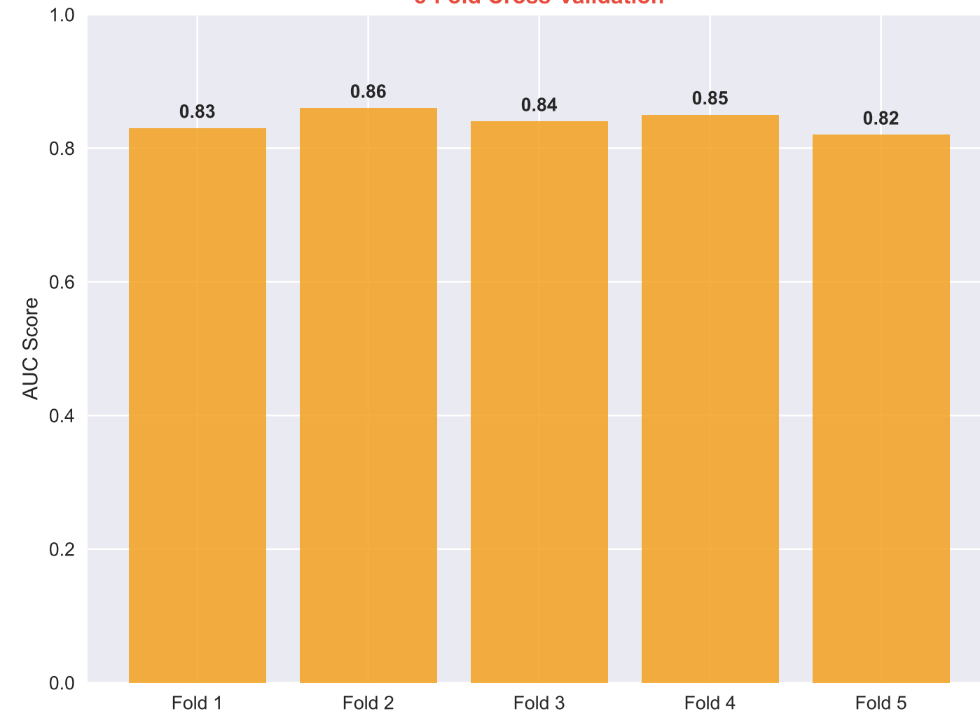
5-Fold Cross-Validation
