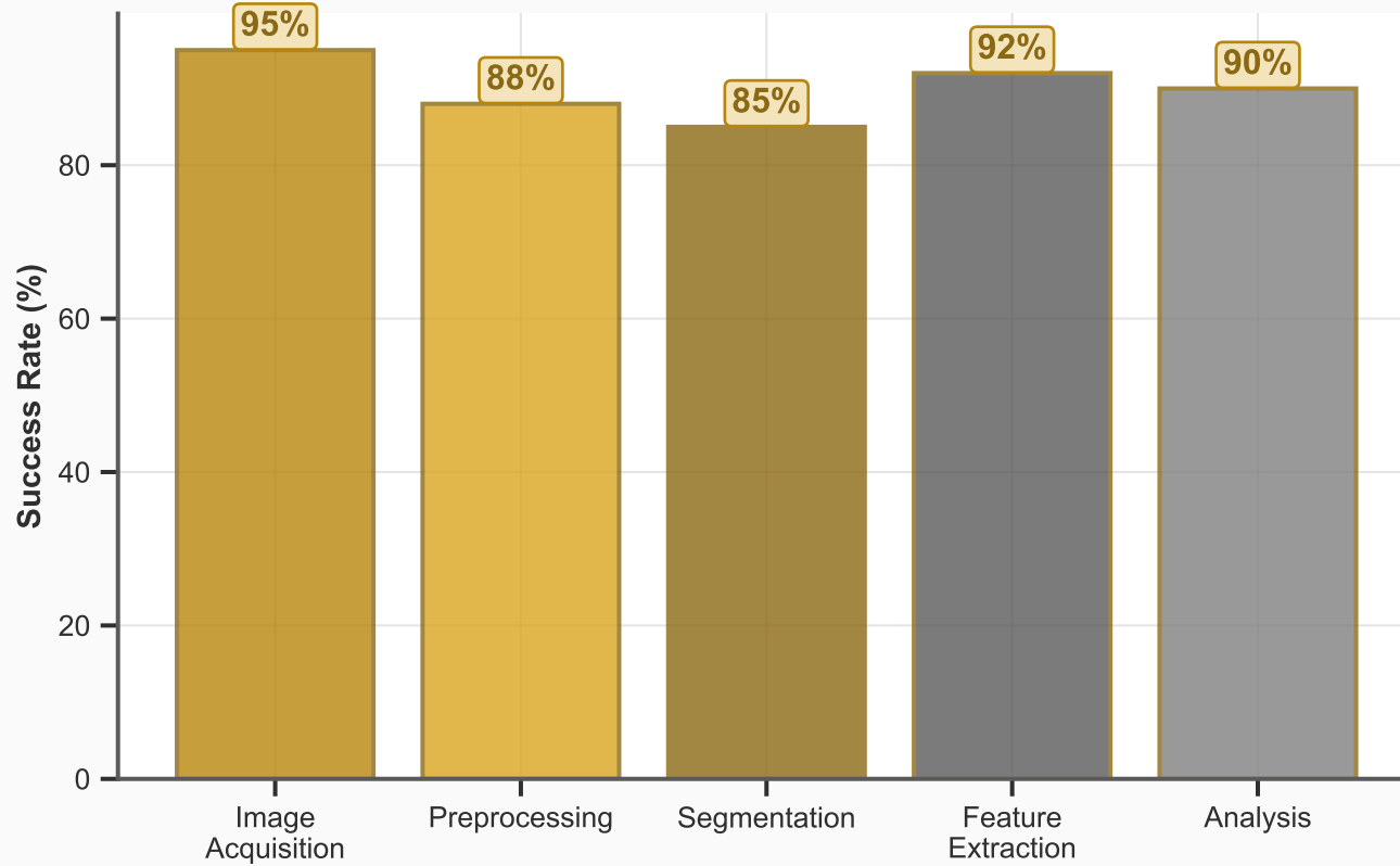
Validation Metrics
