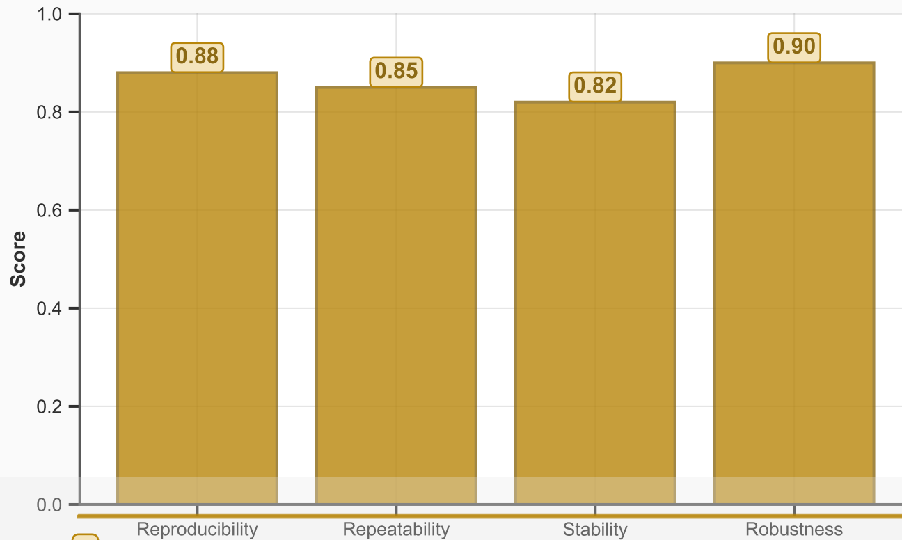
Validation Metrics
