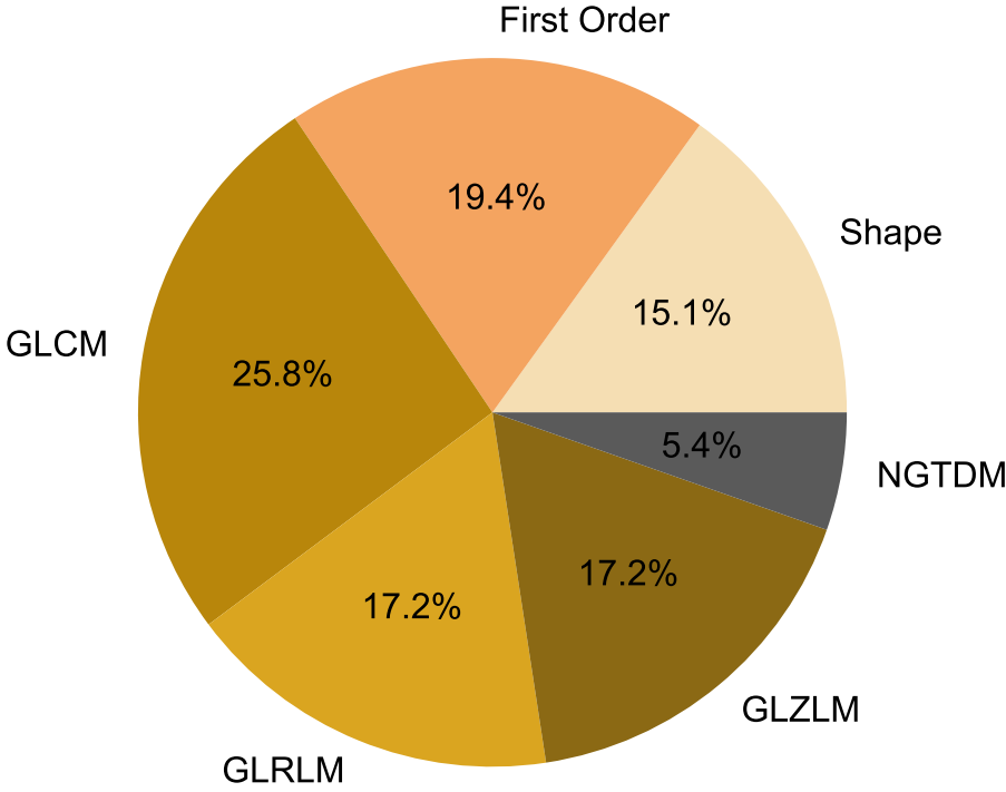
Radiomics Feature Categories
