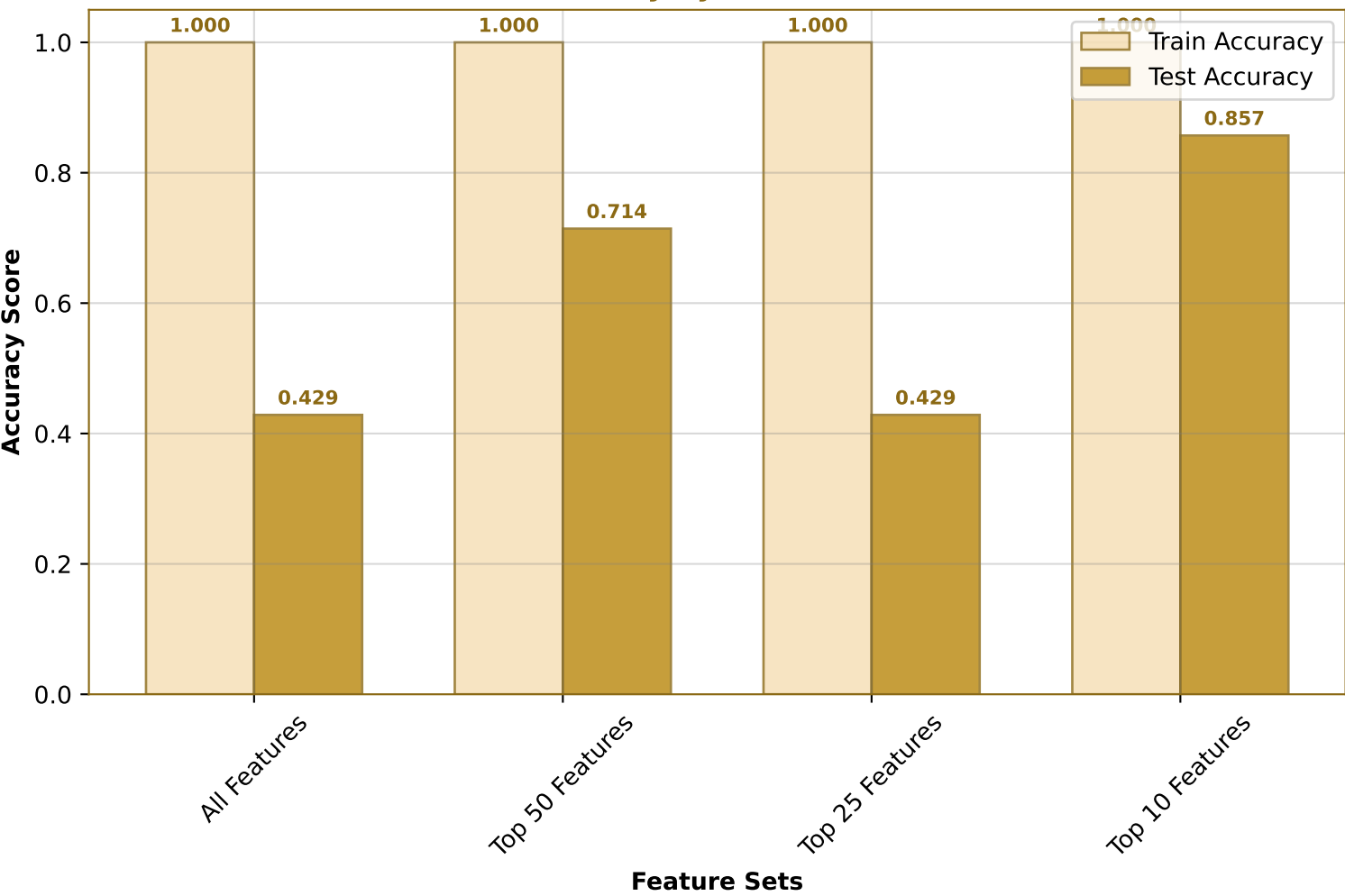
Accuracy by Feature Set
