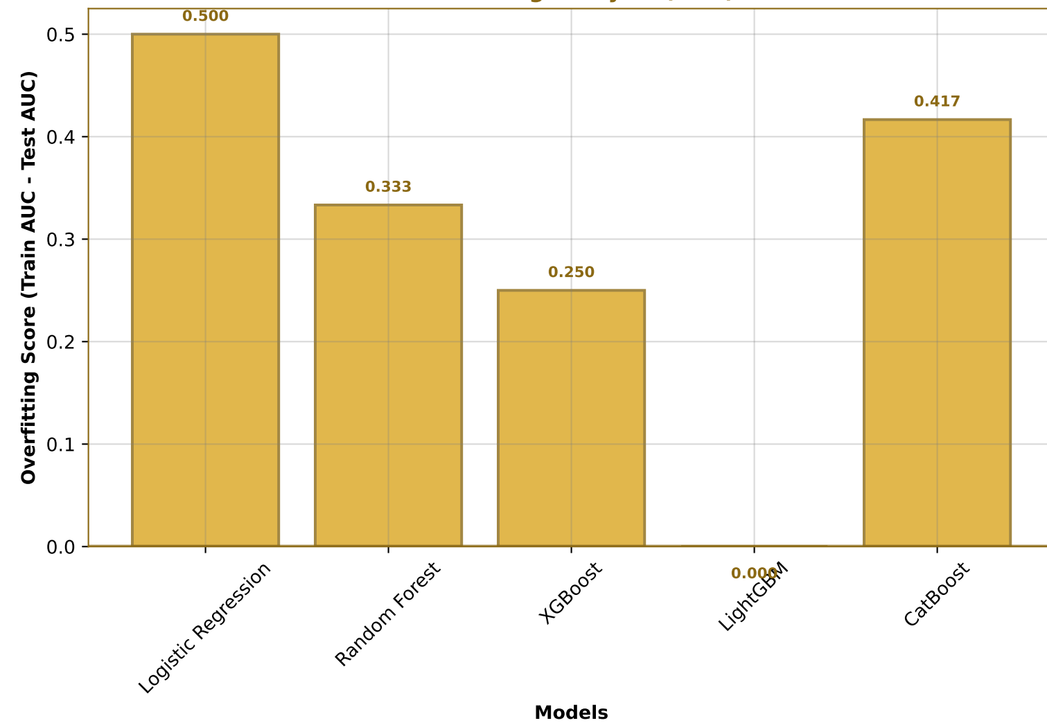
Overfitting Analysis (AUC)
