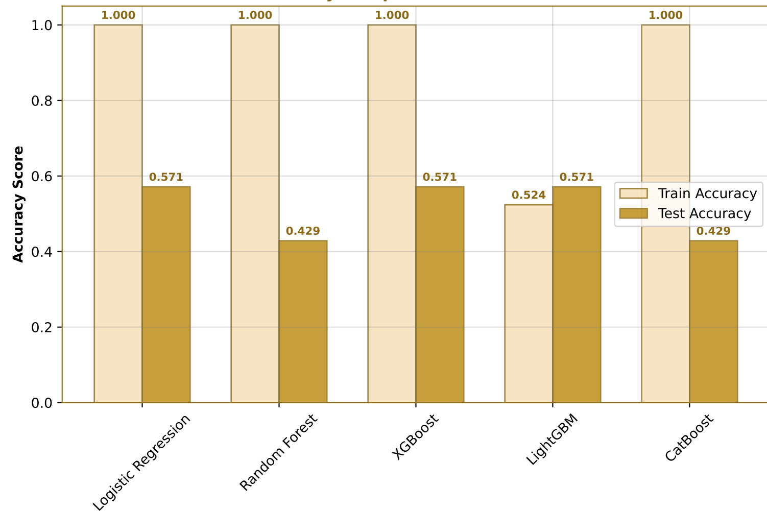
Accuracy Comparison: Train vs Test
