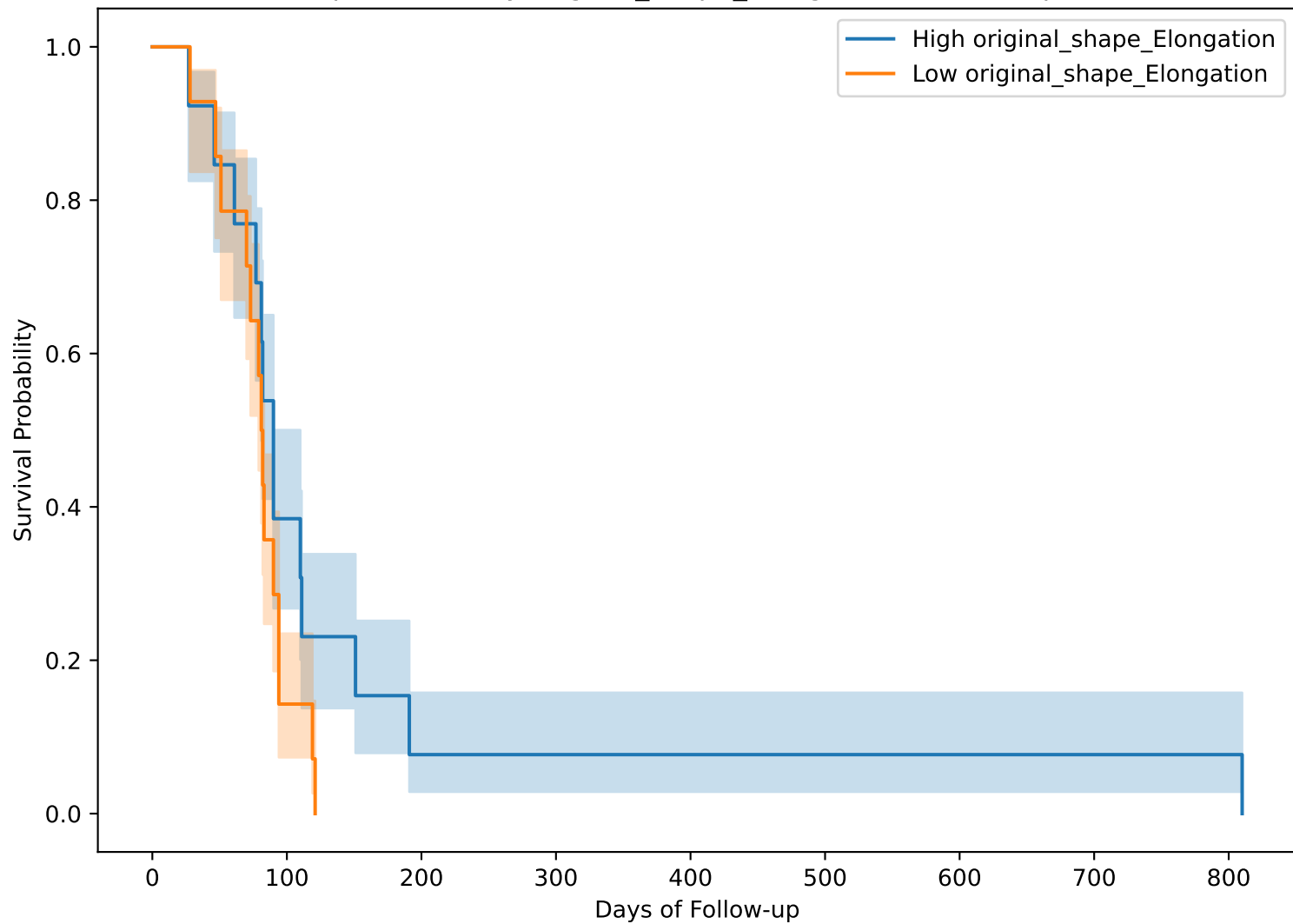
Kaplan-Meier by original_shape_Elongation (median split)
