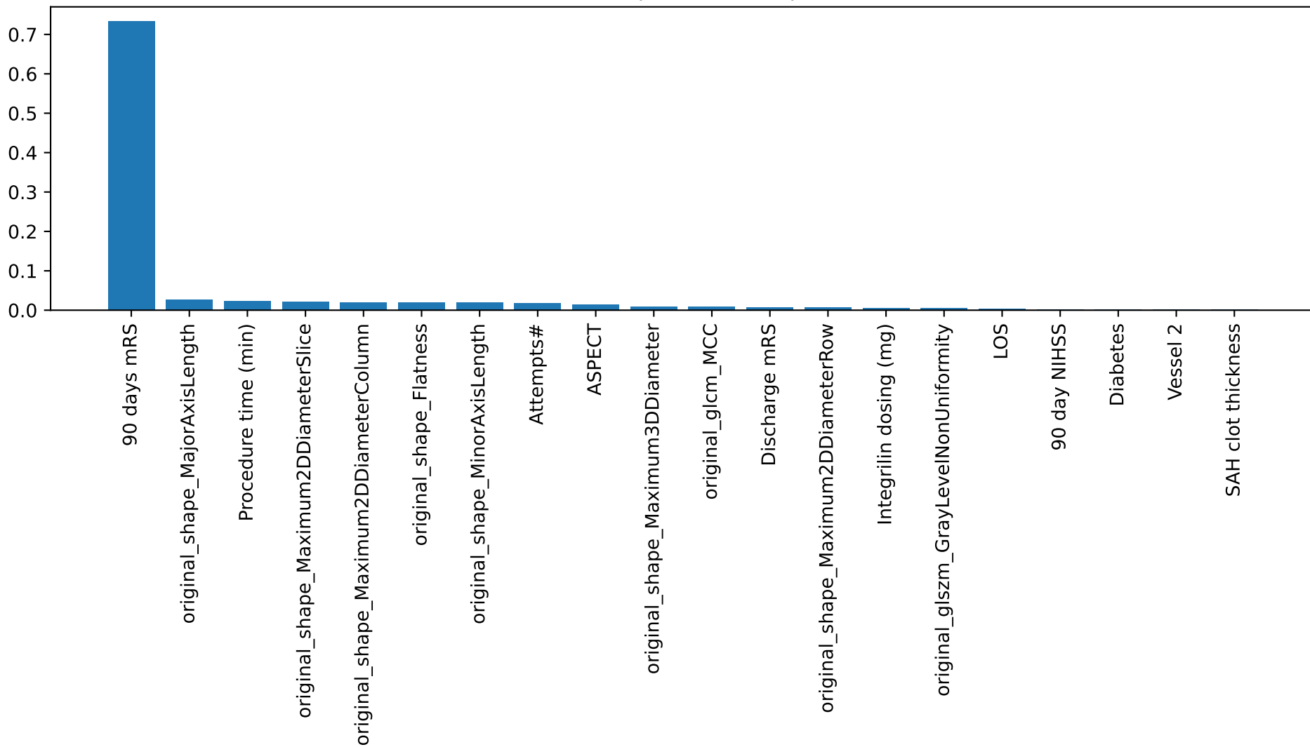
Feature Importances (Top 20)
