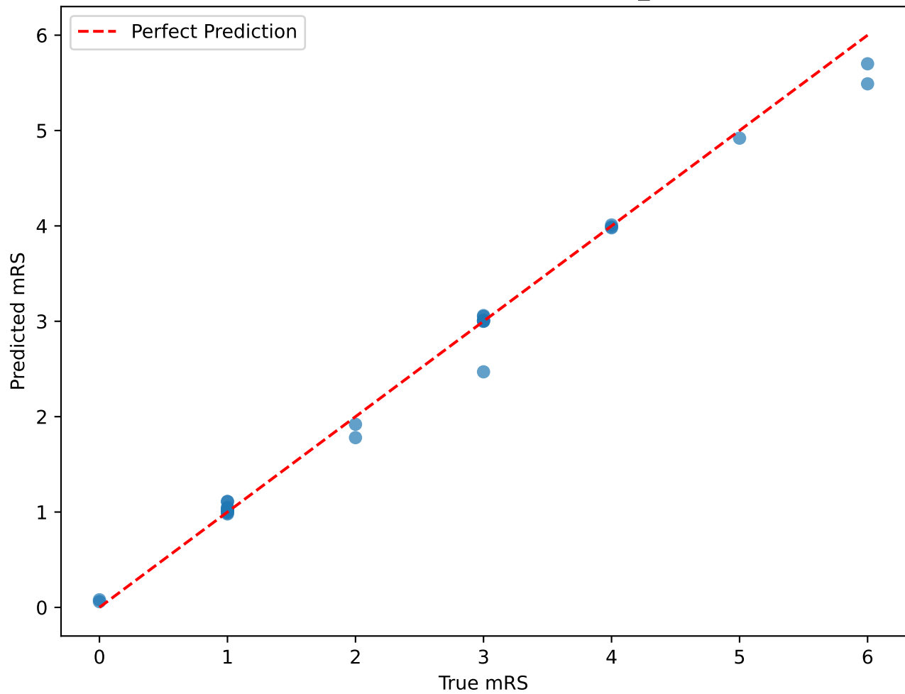
Test: True vs Predicted mRS (2020_2021)
