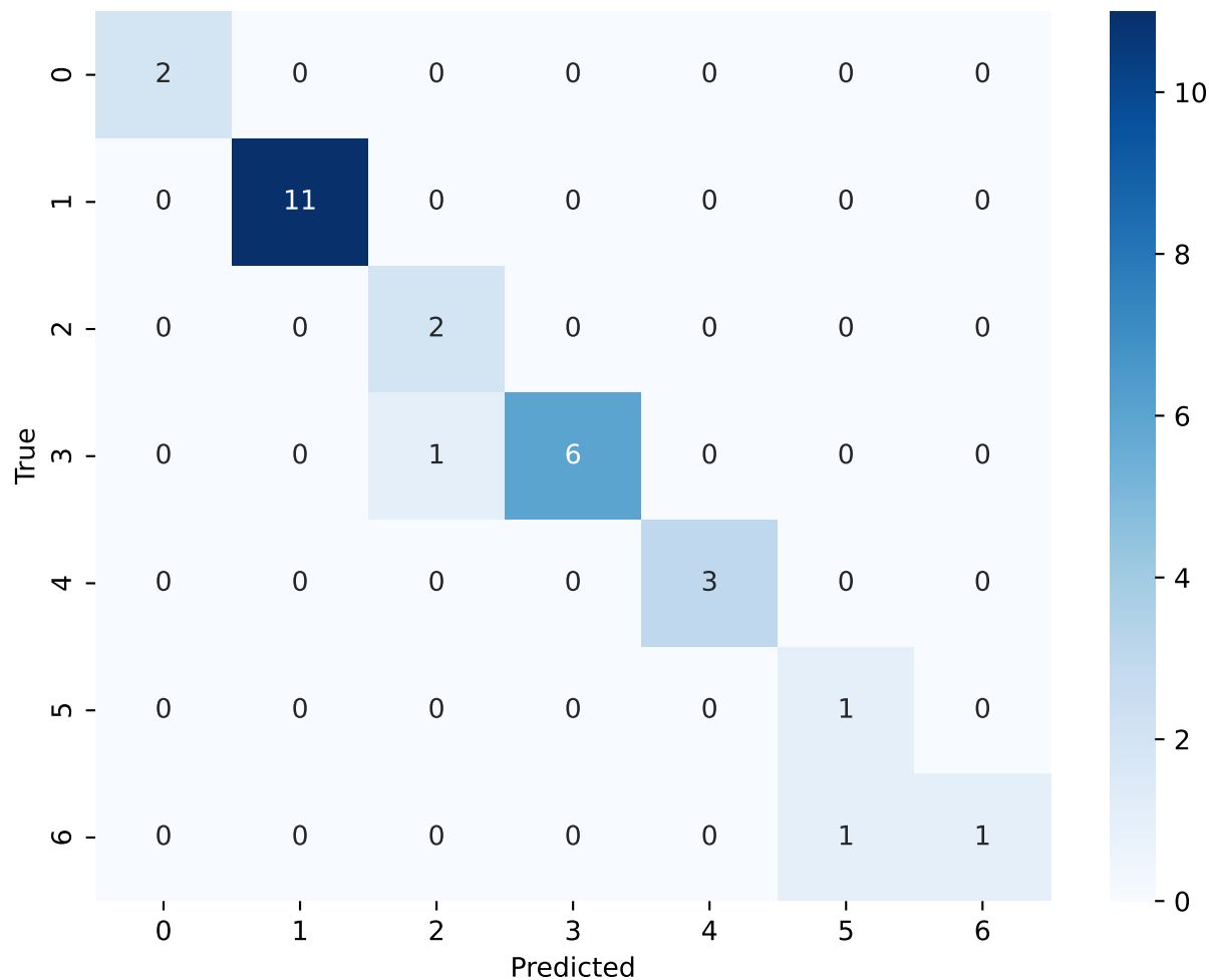
Test Confusion Matrix (rounded mRS)
