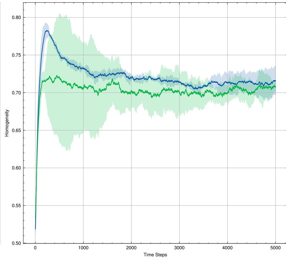
Homogeneity
