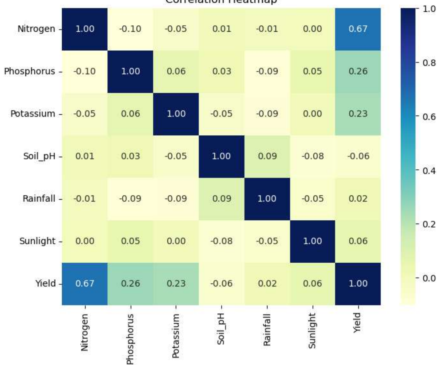
Correlation Heatmap
