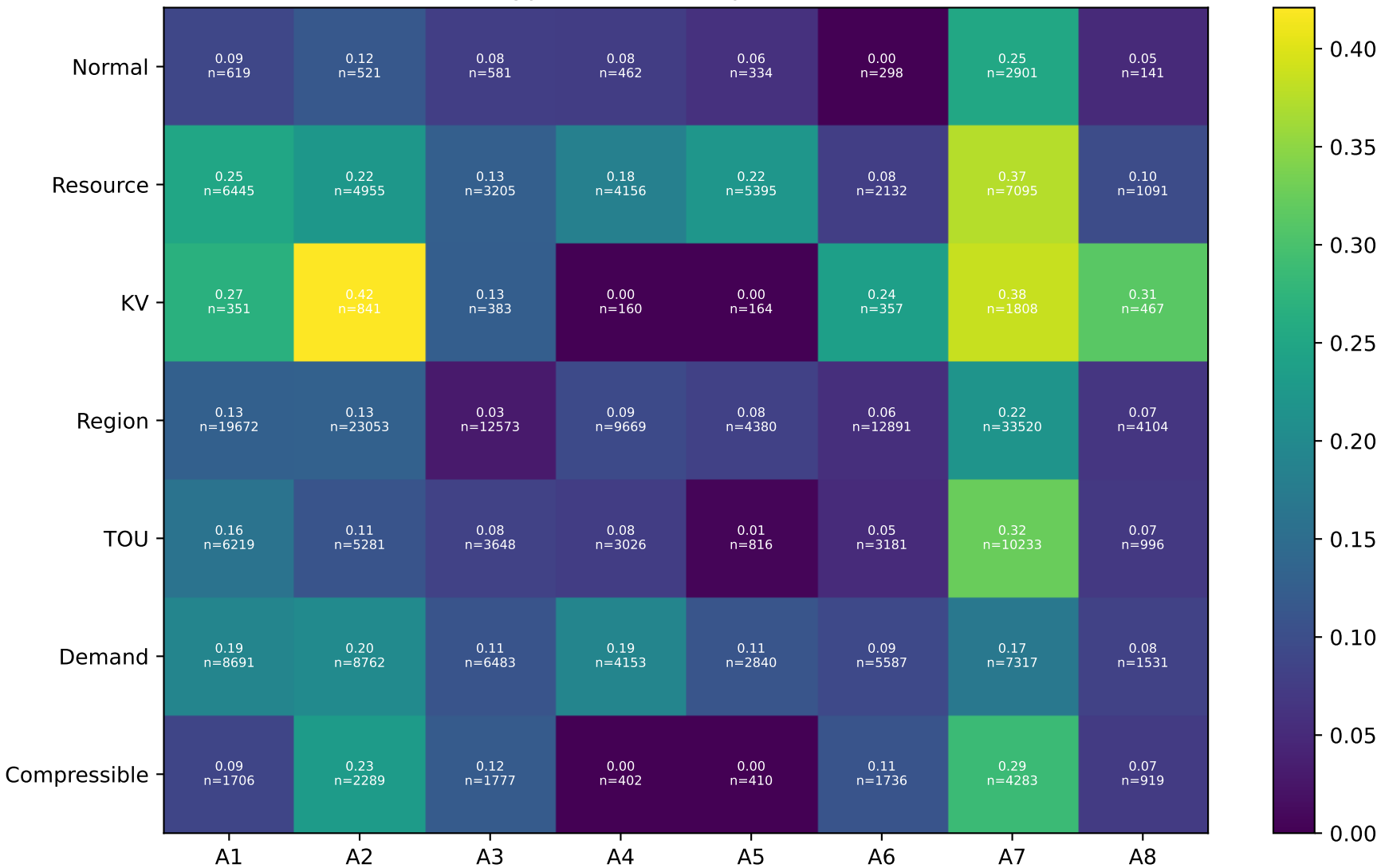
D03 Type-I: Positive improvement rate
