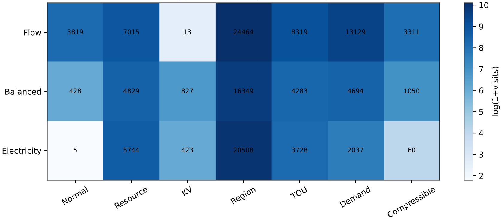
D03 Type-I: Stagnating state coverage
