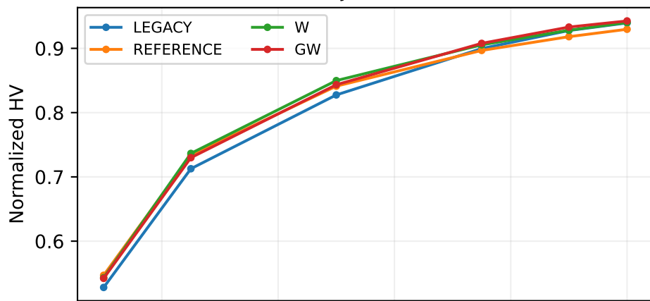
50 jobs / H
