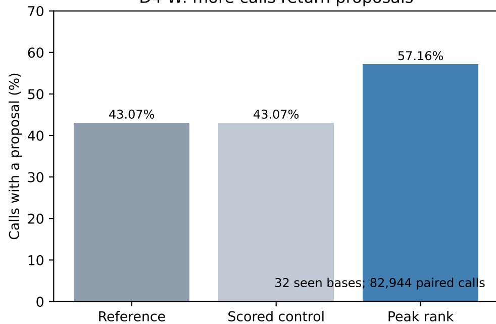
D4-W: more calls return proposals
