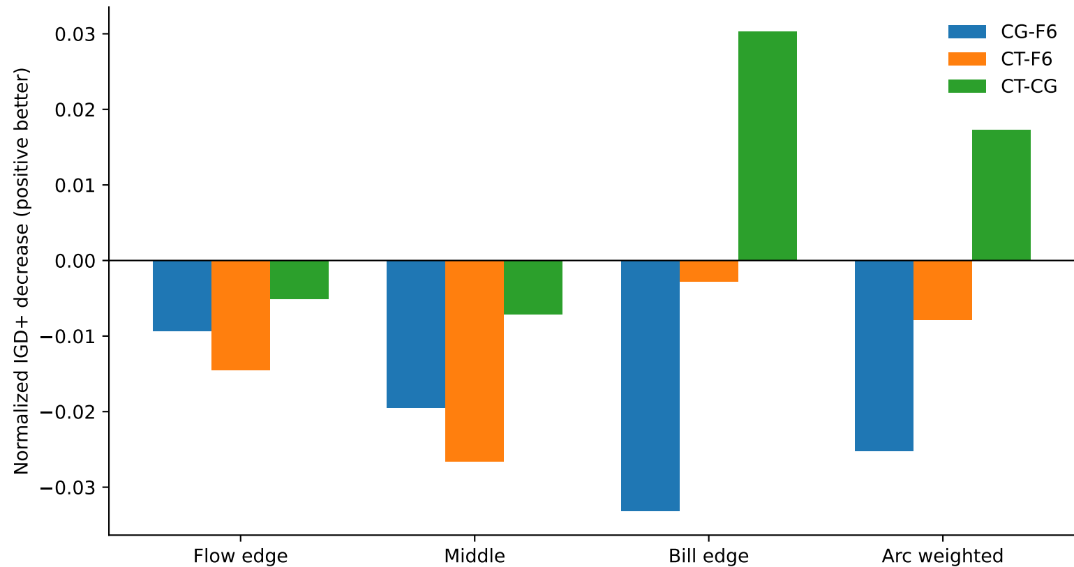
Empirical front coverage: supplementary diagnostics
