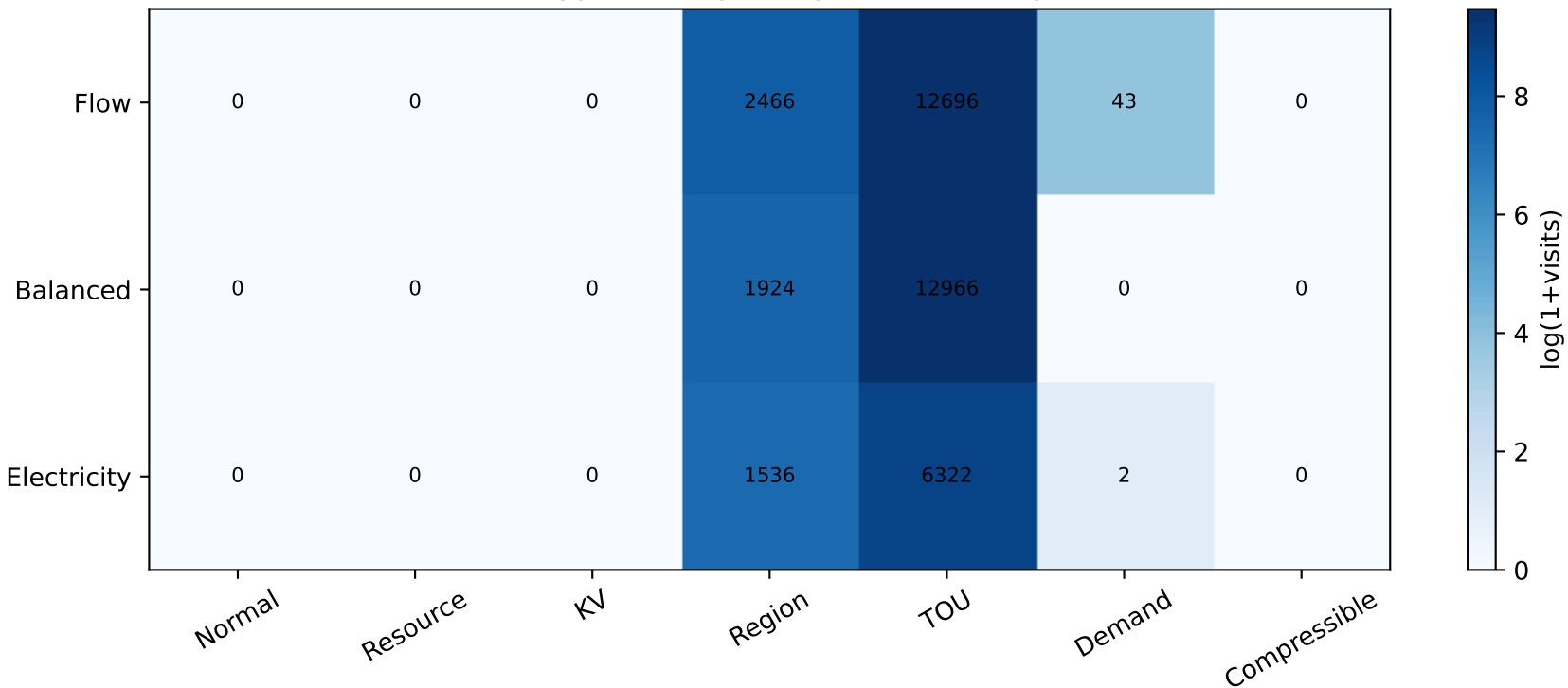
D03 Type-II: Stagnating state coverage
