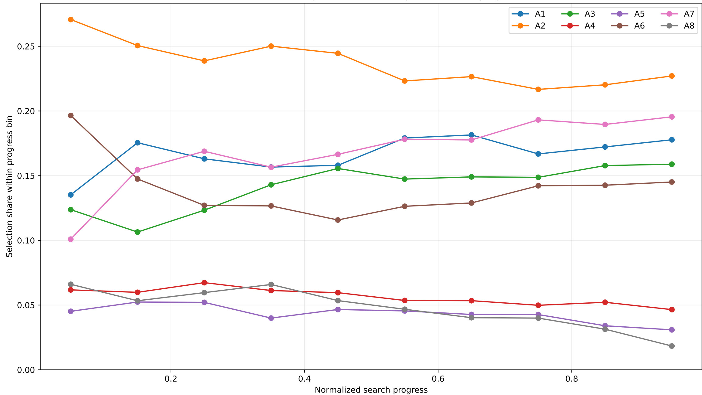
D01 controlled diagnostic: A1-A8 usage over search progress
