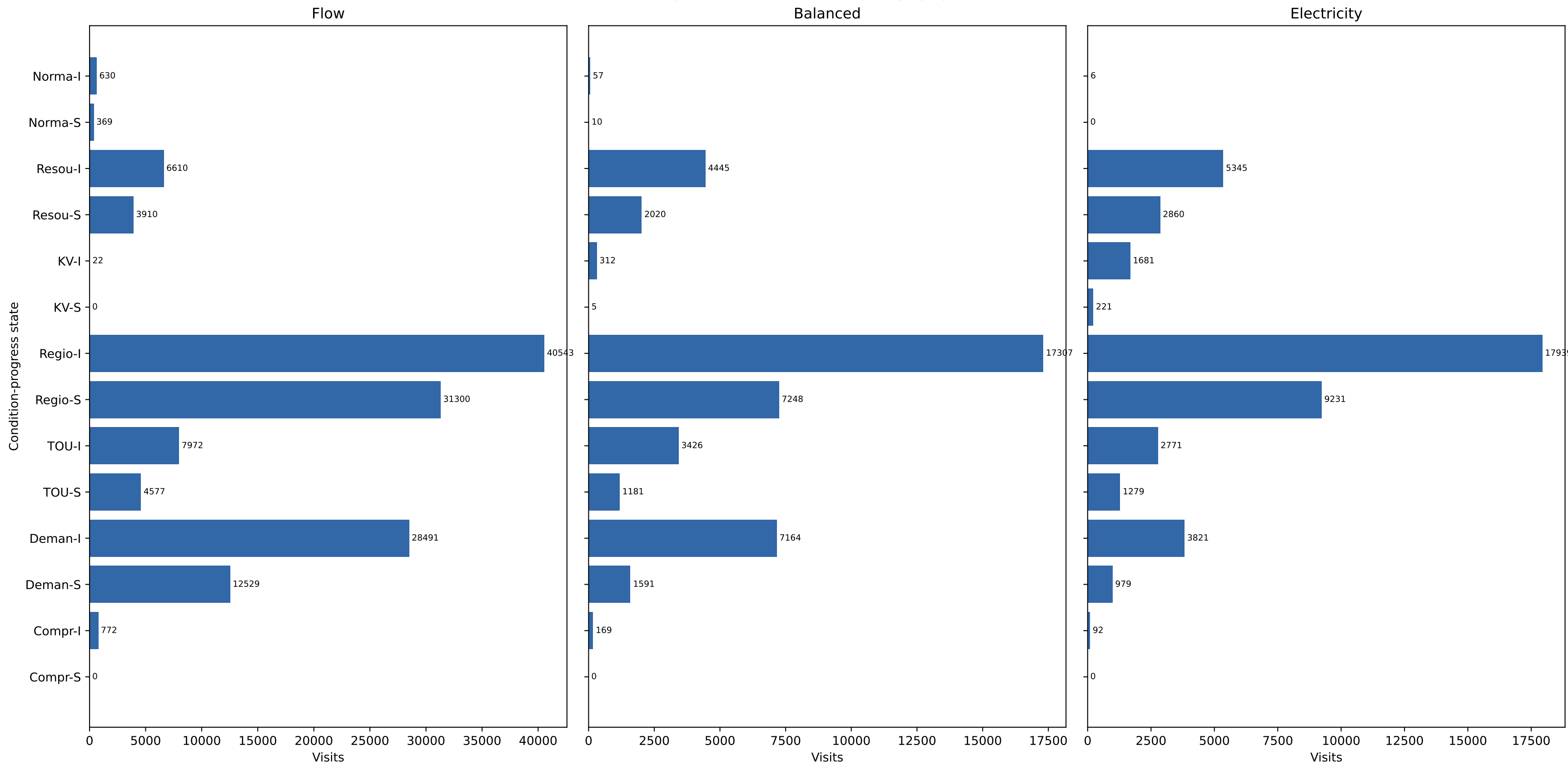
D01 controlled diagnostic: 42-state visit frequency (gray: visits &lt; 30)
