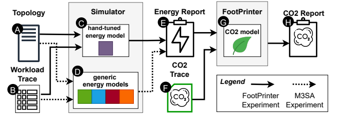
Fig. 8. Overview of experiment 1, adapted and re-run from FootPrinter [16], with M3SA simulation and analysis capabilities.
