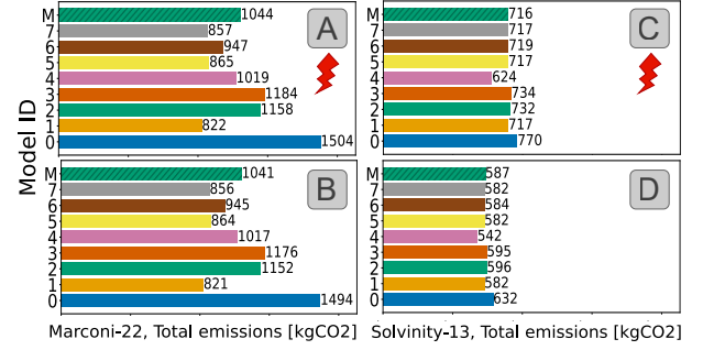
Figure 12: Total emissions generated by a workload trace running in S2. Left column, Marconi-22 workload: (A) S2 experiences Ldns04-based failures, (B) S2 without failures. Right column, Solvinty-13 workload: (C) S2 experiences Ldns04-based failures, (D) S2 without failures. Each plot shows the total CO2 emissions predicted by the M3SA Multi-Model using eight generic energy-models (labeled 0-7) and by the Meta-Model (M).
