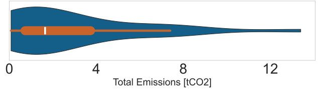
Fig. 14. Total CO2 emitted when running the Marconi-22 workload on S3, assessed for 29 European countries, as of June 2023.
