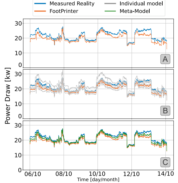
Fig. 9. Simulation results vs. measured reality: (A) FootPrinter simulator, peer-reviewed experiment [16]; (B) Multi-Model with four individual models vs. FootPrinter; (C) Meta-Model derived from the Multi-Model at point B.
