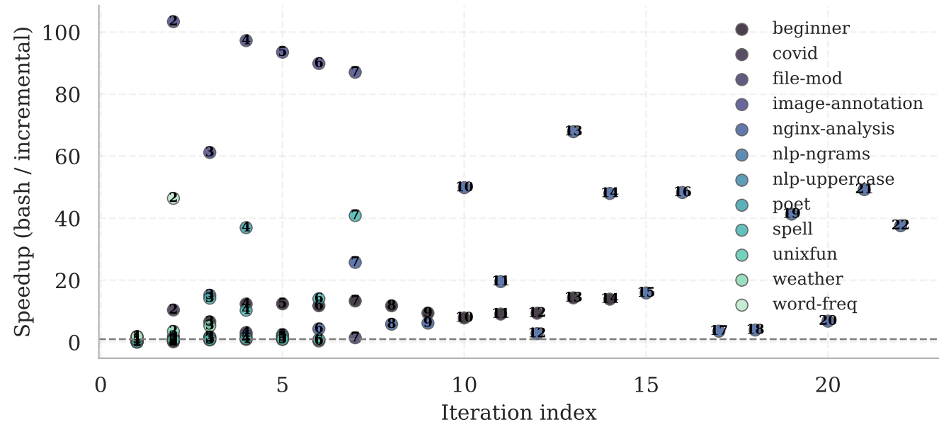
Per-iteration Speedup Across Benchmarks
